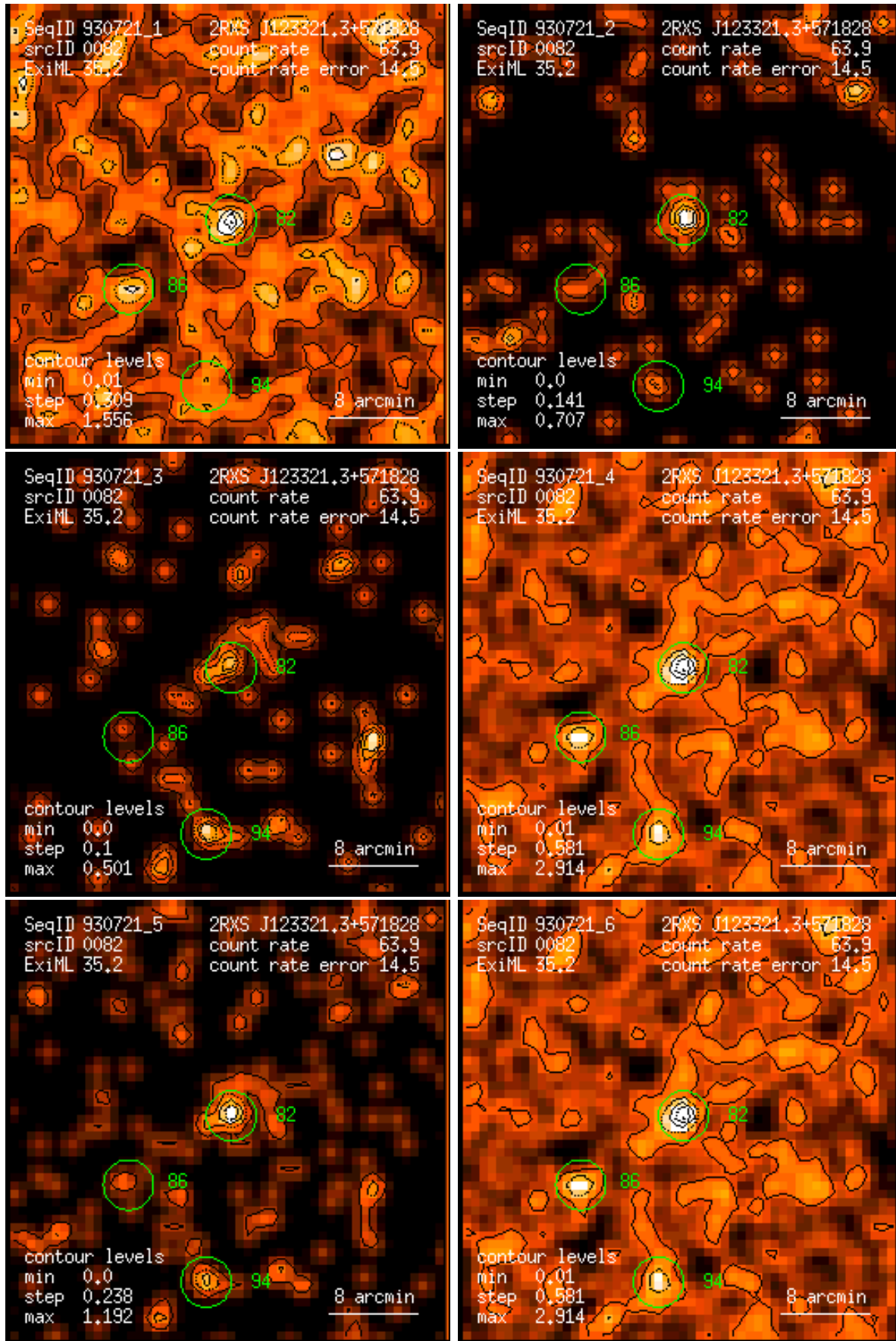
Figure 82: RASS 930721: detection 0082: band rate images, Gaussian filter: (1) PSPC channels 11 – 41, (2) 52 – 90, (3) 91 – 201, (4) 11 – 235, (5) 52 – 201, (6) 11 – 201. Broad band rates in counts/ks. Band rate contour levels in counts/ks/arcmin 2 .
