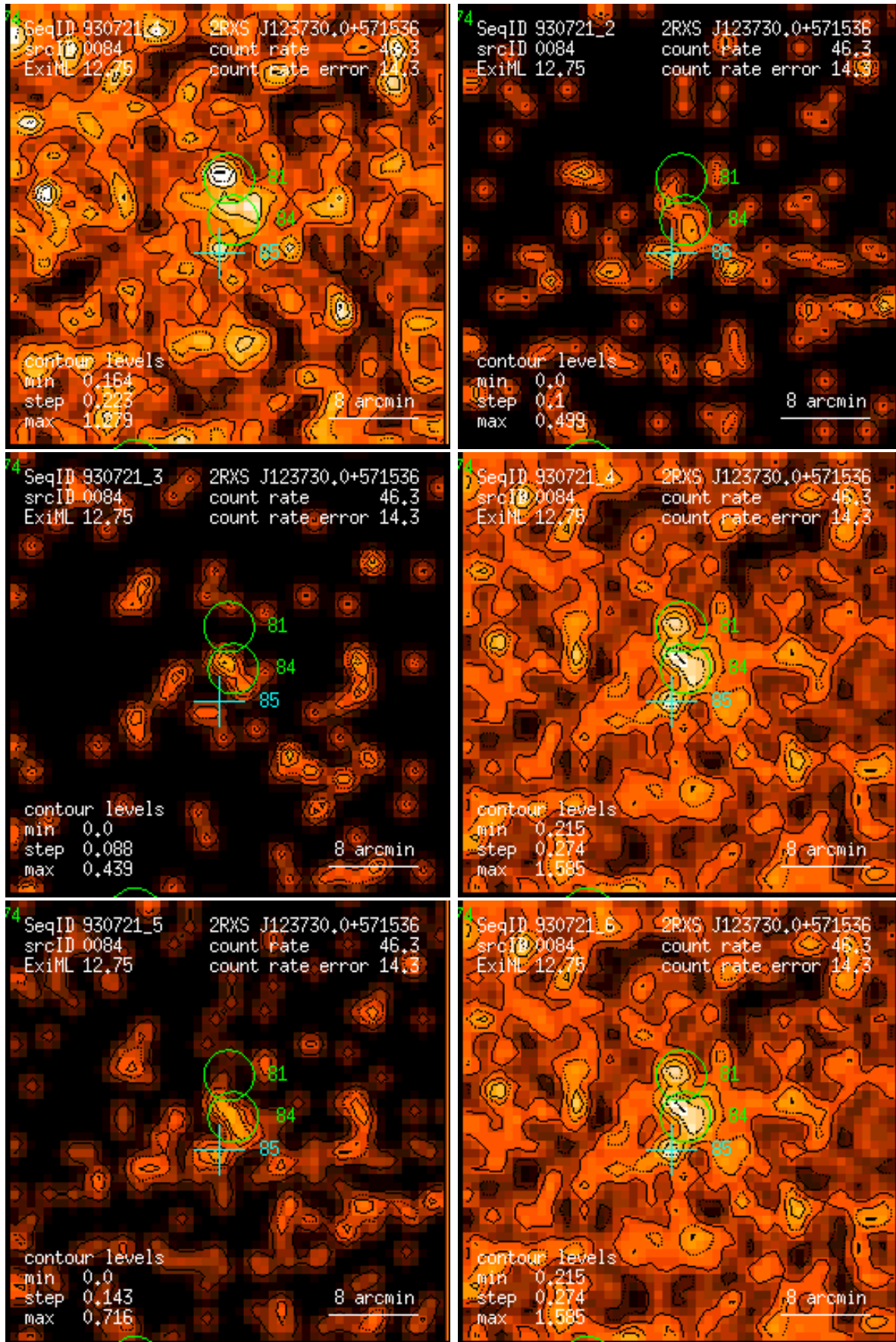
Figure 84: RASS 930721: detection 0084: band rate images, Gaussian filter: (1) PSPC channels 11 – 41, (2) 52 – 90, (3) 91 – 201, (4) 11 – 235, (5) 52 – 201, (6) 11 – 201. Broad band rates in counts/ks. Band rate contour levels in counts/ks/arcmin 2 .
