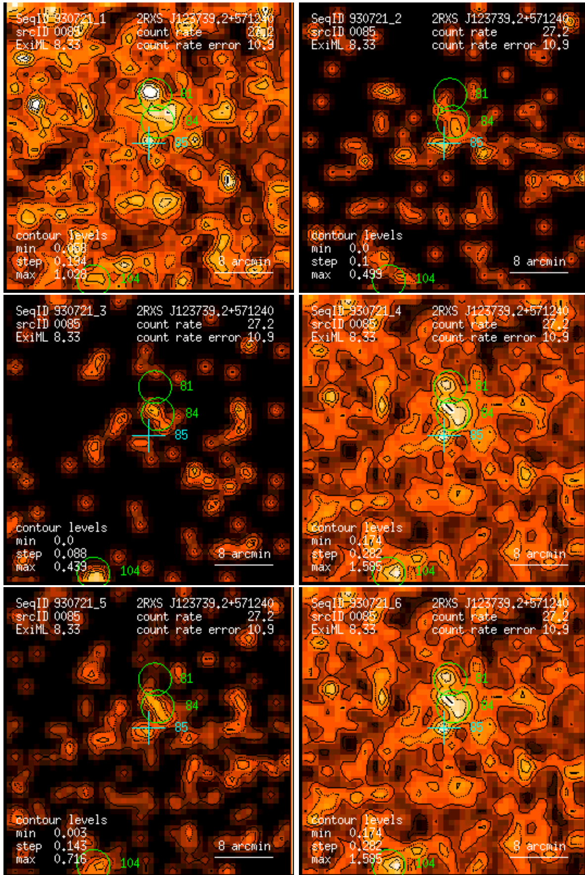
Figure 85: RASS 930721: detection 0085: band rate images, Gaussian filter: (1) PSPC channels 11 – 41, (2) 52 – 90, (3) 91 – 201, (4) 11 – 235, (5) 52 – 201, (6) 11 – 201. Broad band rates in counts/ks. Band rate contour levels in counts/ks/arcmin 2 .
