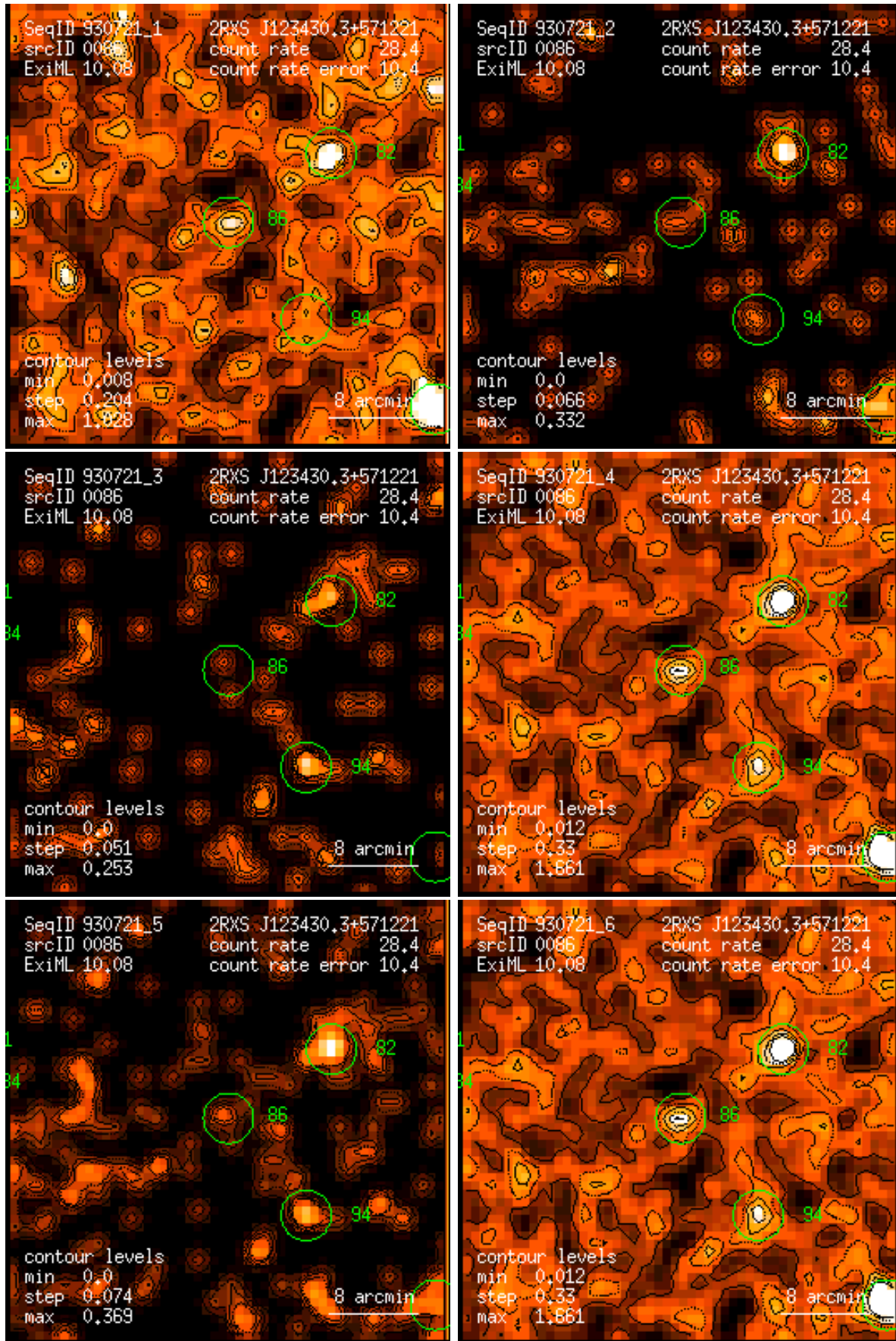
Figure 86: RASS 930721: detection 0086: band rate images, Gaussian filter: (1) PSPC channels 11 – 41, (2) 52 – 90, (3) 91 – 201, (4) 11 – 235, (5) 52 – 201, (6) 11 – 201. Broad band rates in counts/ks. Band rate contour levels in counts/ks/arcmin 2 .
