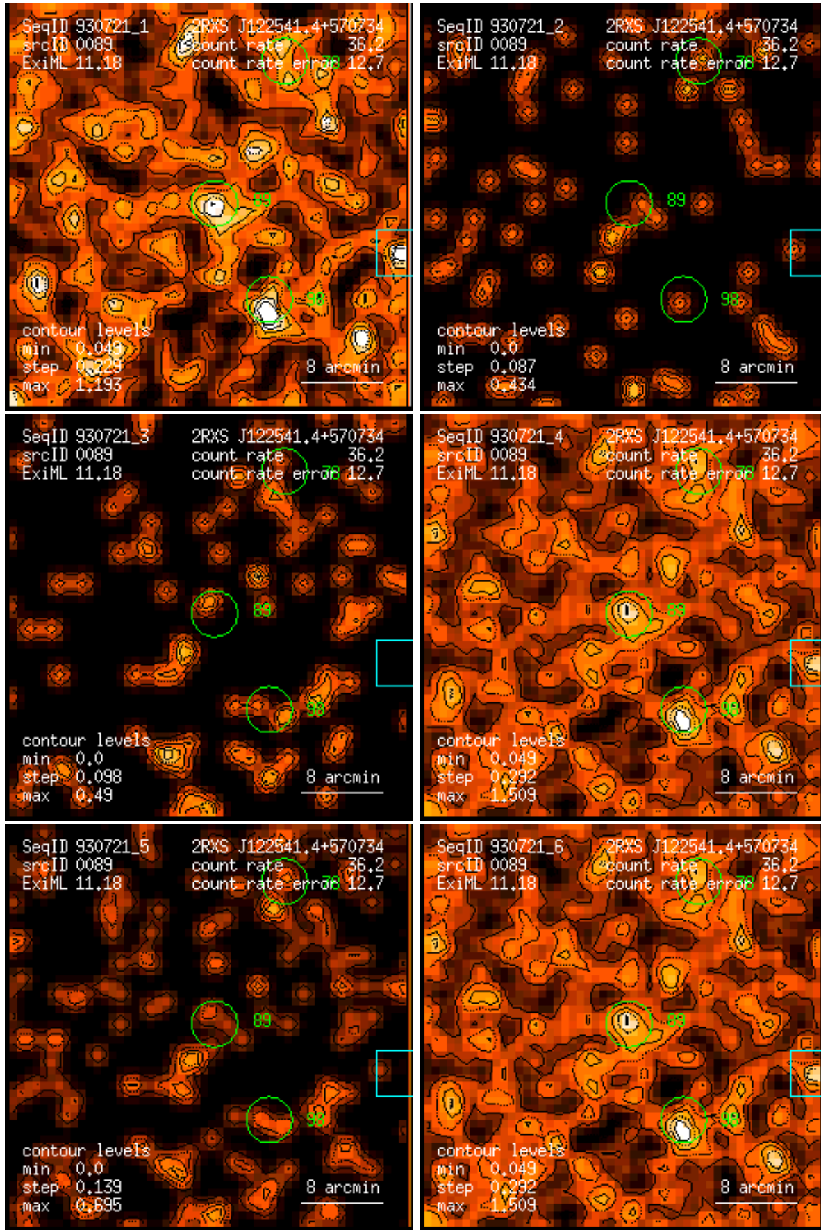
Figure 89: RASS 930721: detection 0089: band rate images, Gaussian filter: (1) PSPC channels 11 – 41, (2) 52 – 90, (3) 91 – 201, (4) 11 – 235, (5) 52 – 201, (6) 11 – 201. Broad band rates in counts/ks. Band rate contour levels in counts/ks/arcmin 2 .
