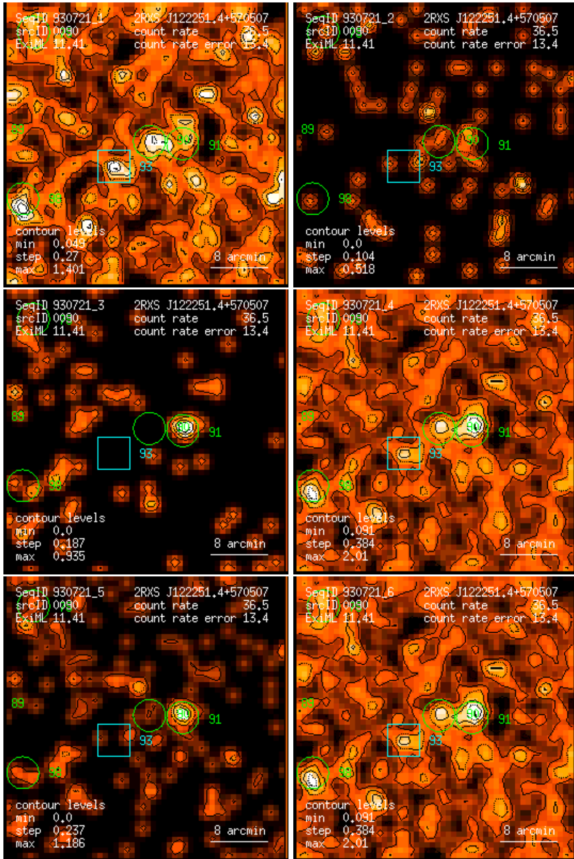
Figure 90: RASS 930721: detection 0090: band rate images, Gaussian filter: (1) PSPC channels 11 – 41, (2) 52 – 90, (3) 91 – 201, (4) 11 – 235, (5) 52 – 201, (6) 11 – 201. Broad band rates in counts/ks. Band rate contour levels in counts/ks/arcmin 2 .
