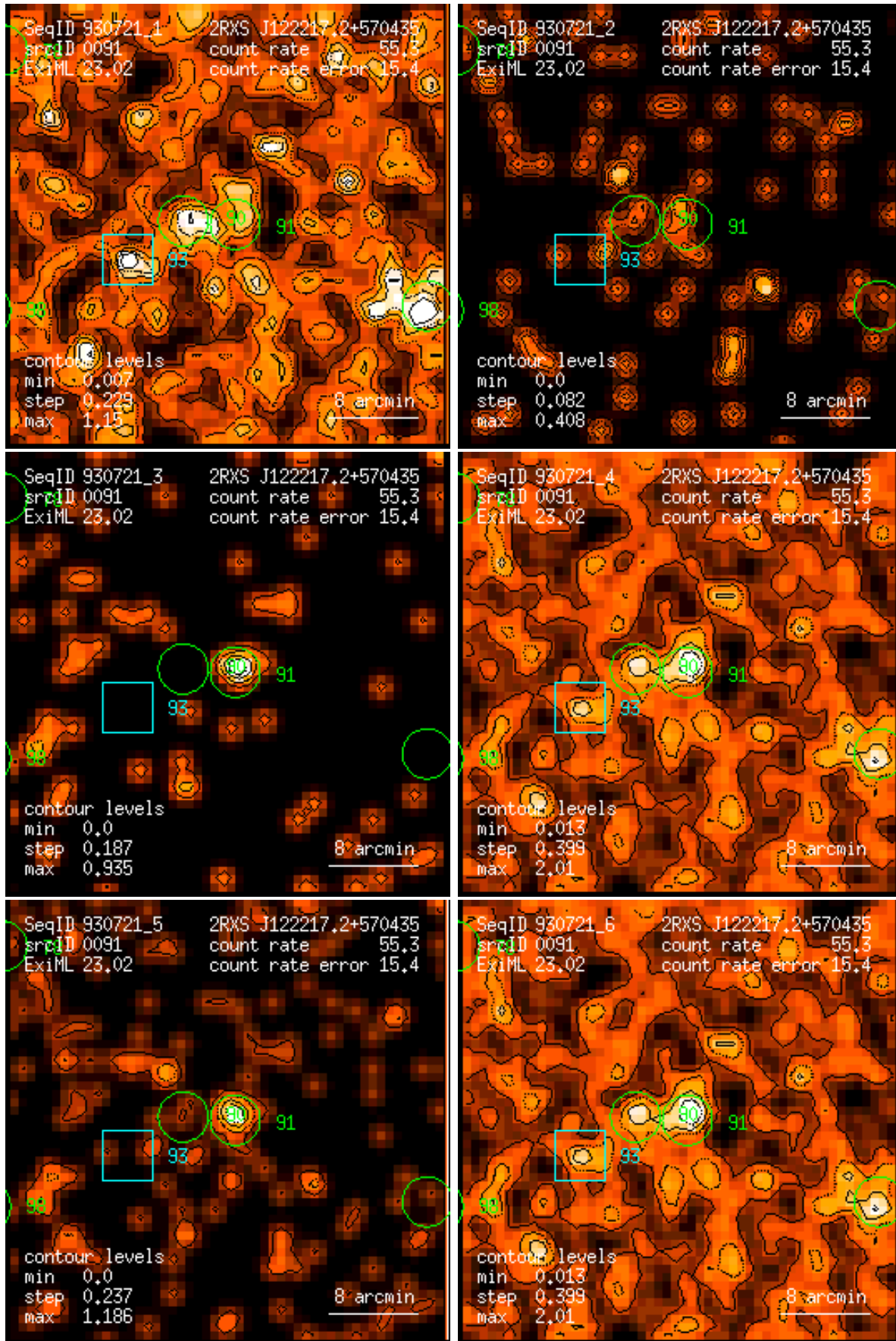
Figure 91: RASS 930721: detection 0091: band rate images, Gaussian filter: (1) PSPC channels 11 – 41, (2) 52 – 90, (3) 91 – 201, (4) 11 – 235, (5) 52 – 201, (6) 11 – 201. Broad band rates in counts/ks. Band rate contour levels in counts/ks/arcmin 2 .
