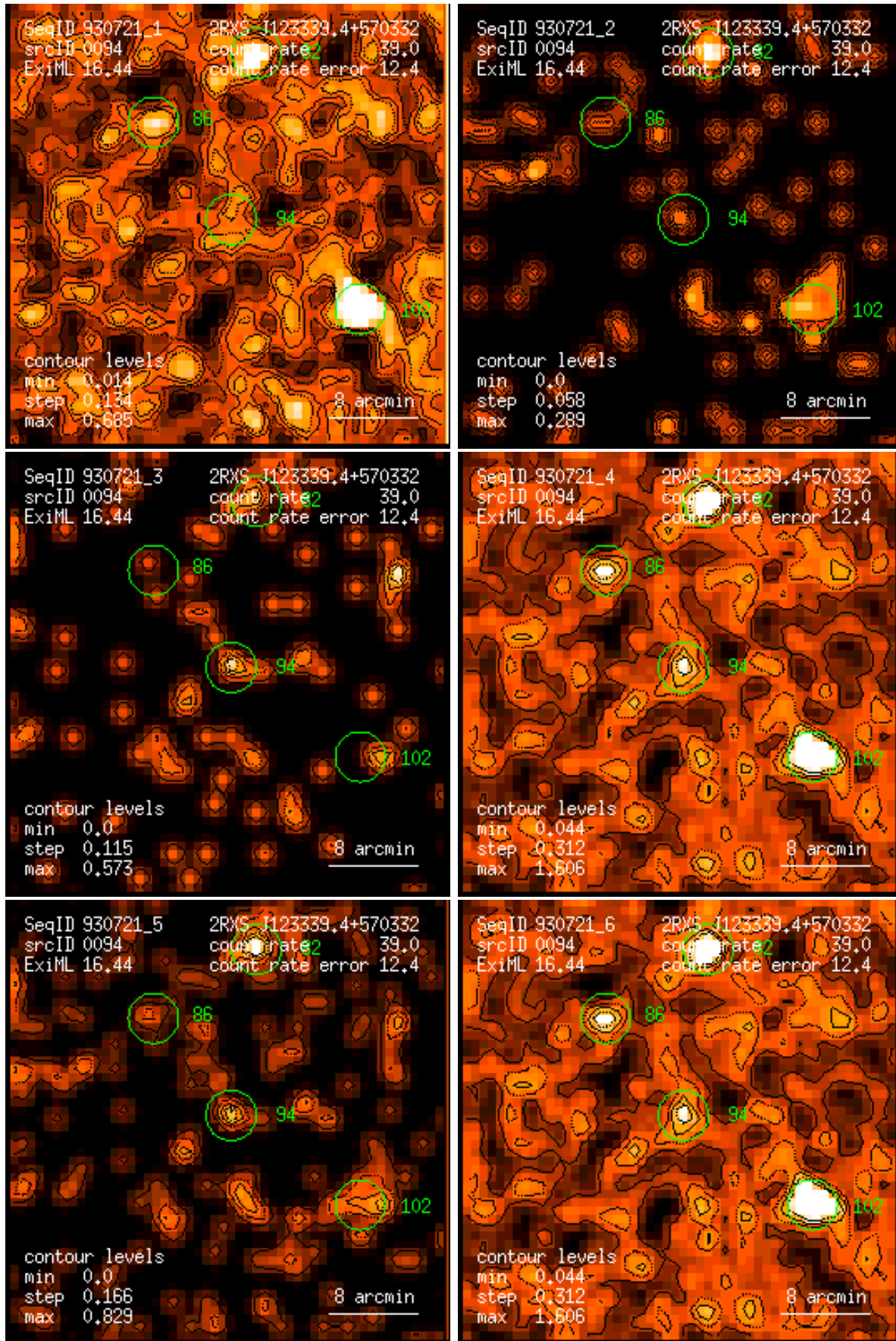
Figure 94: RASS 930721: detection 0094: band rate images, Gaussian filter: (1) PSPC channels 11 – 41, (2) 52 – 90, (3) 91 – 201, (4) 11 – 235, (5) 52 – 201, (6) 11 – 201. Broad band rates in counts/ks. Band rate contour levels in counts/ks/arcmin 2 .
