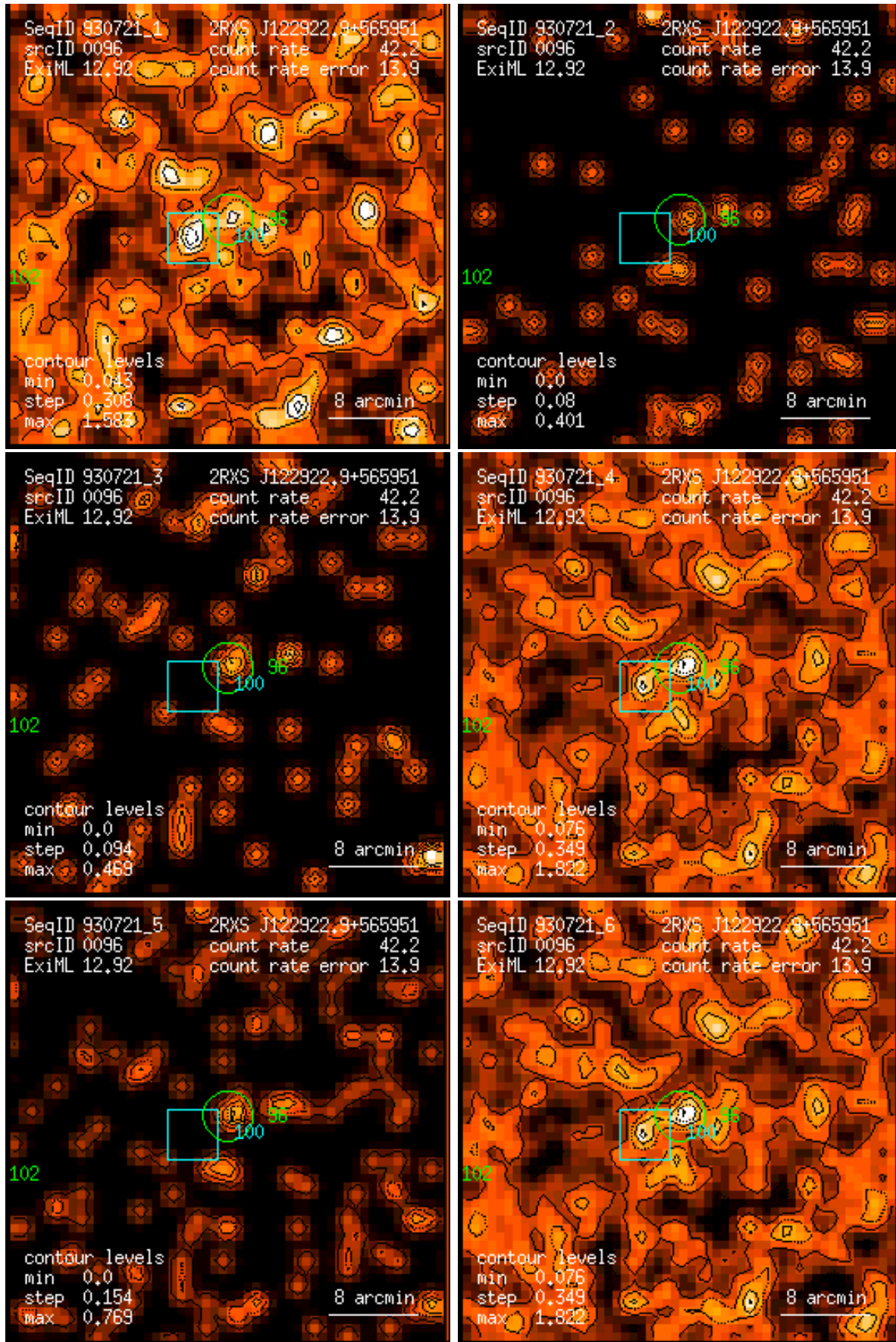
Figure 96: RASS 930721: detection 0096: band rate images, Gaussian filter: (1) PSPC channels 11 – 41, (2) 52 – 90, (3) 91 – 201, (4) 11 – 235, (5) 52 – 201, (6) 11 – 201. Broad band rates in counts/ks. Band rate contour levels in counts/ks/arcmin 2 .
