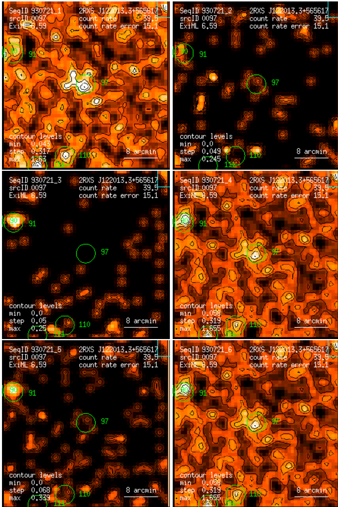
Figure 97: RASS 930721: detection 0097: band rate images, Gaussian filter: (1) PSPC channels 11 – 41, (2) 52 – 90, (3) 91 – 201, (4) 11 – 235, (5) 52 – 201, (6) 11 – 201. Broad band rates in counts/ks. Band rate contour levels in counts/ks/arcmin 2 .
