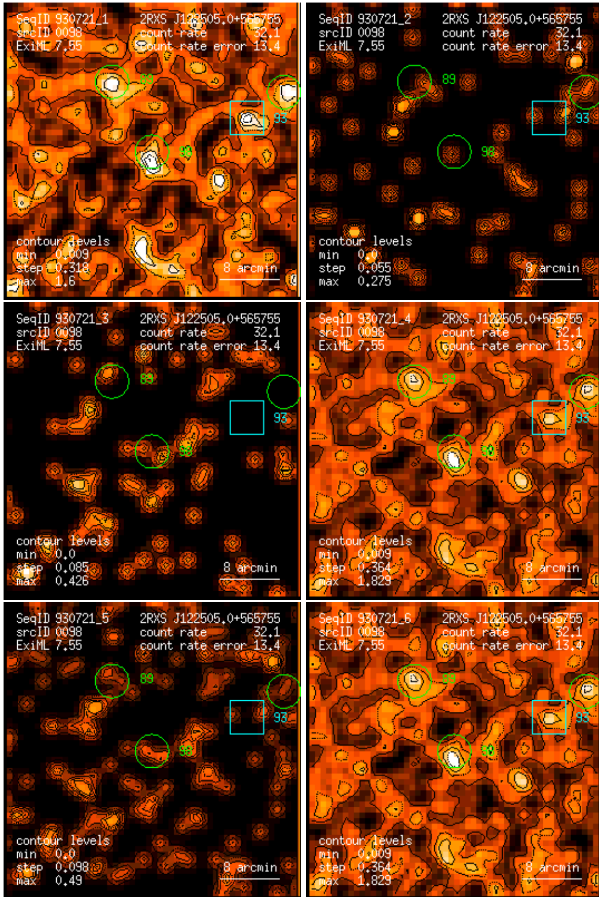
Figure 98: RASS 930721: detection 0098: band rate images, Gaussian filter: (1) PSPC channels 11 – 41, (2) 52 – 90, (3) 91 – 201, (4) 11 – 235, (5) 52 – 201, (6) 11 – 201. Broad band rates in counts/ks. Band rate contour levels in counts/ks/arcmin 2 .
