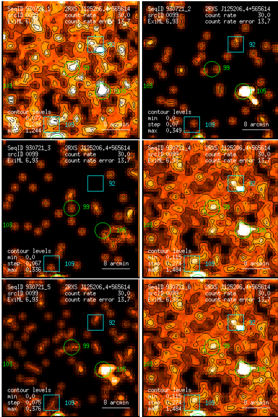
Figure 99: RASS 930721: detection 0099: band rate images, Gaussian filter: (1) PSPC channels 11 – 41, (2) 52 – 90, (3) 91 – 201, (4) 11 – 235, (5) 52 – 201, (6) 11 – 201. Broad band rates in counts/ks. Band rate contour levels in counts/ks/arcmin 2 .
