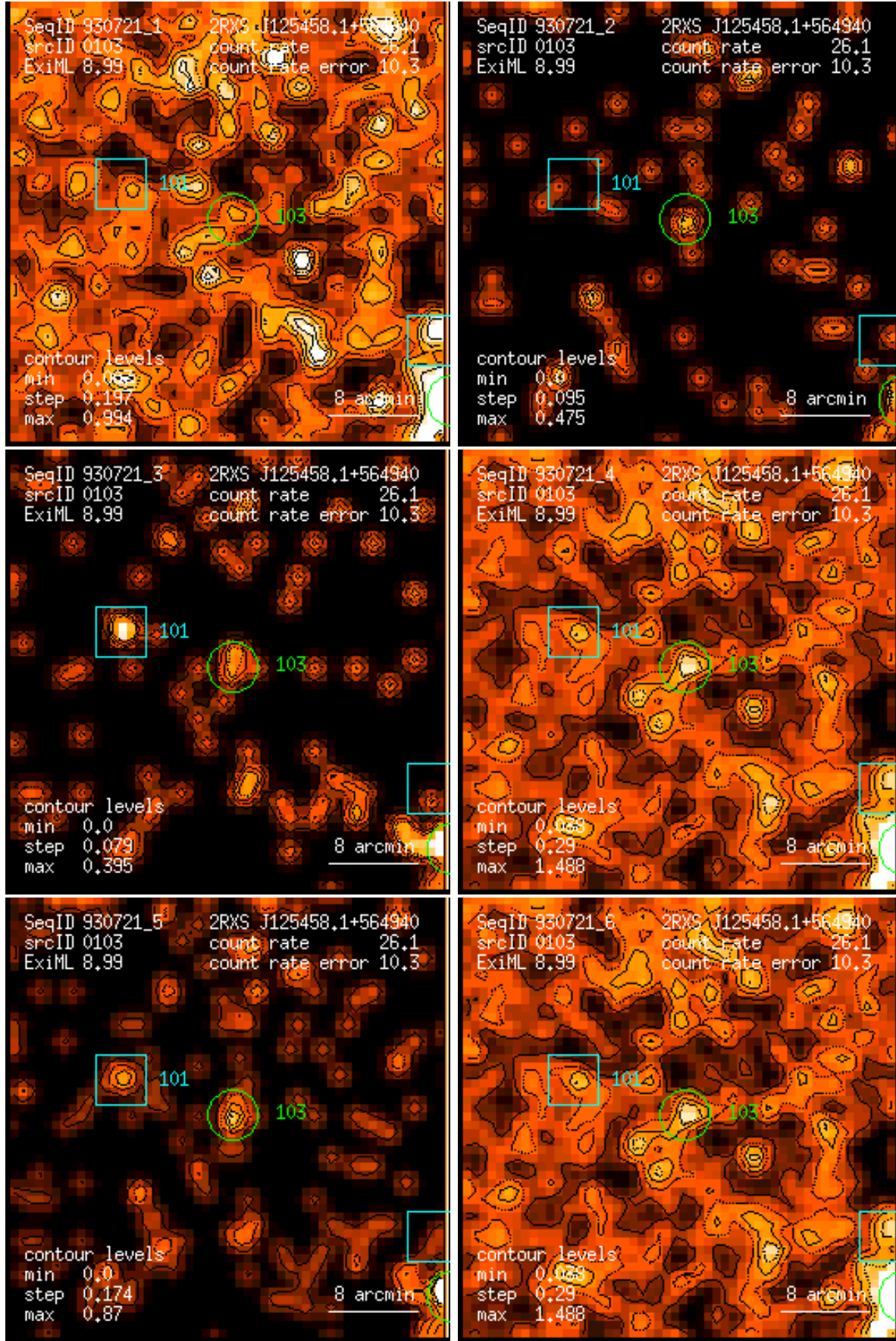
Figure 103: RASS 930721: detection 0103: band rate images, Gaussian filter: (1) PSPC channels 11 – 41, (2) 52 – 90, (3) 91 – 201, (4) 11 – 235, (5) 52 – 201, (6) 11 – 201. Broad band rates in counts/ks. Band rate contour levels in counts/ks/arcmin 2 .
