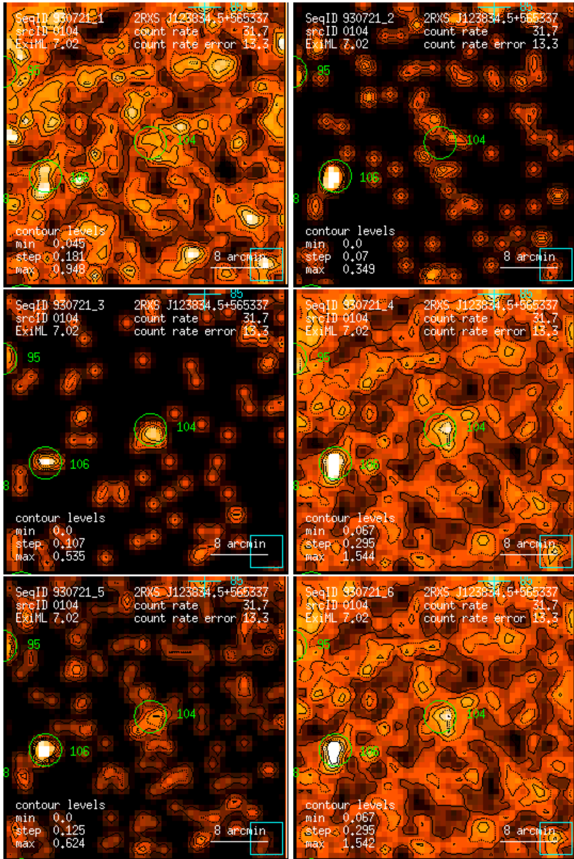
Figure 104: RASS 930721: detection 0104: band rate images, Gaussian filter: (1) PSPC channels 11 – 41, (2) 52 – 90, (3) 91 – 201, (4) 11 – 235, (5) 52 – 201, (6) 11 – 201. Broad band rates in counts/ks. Band rate contour levels in counts/ks/arcmin 2 .
