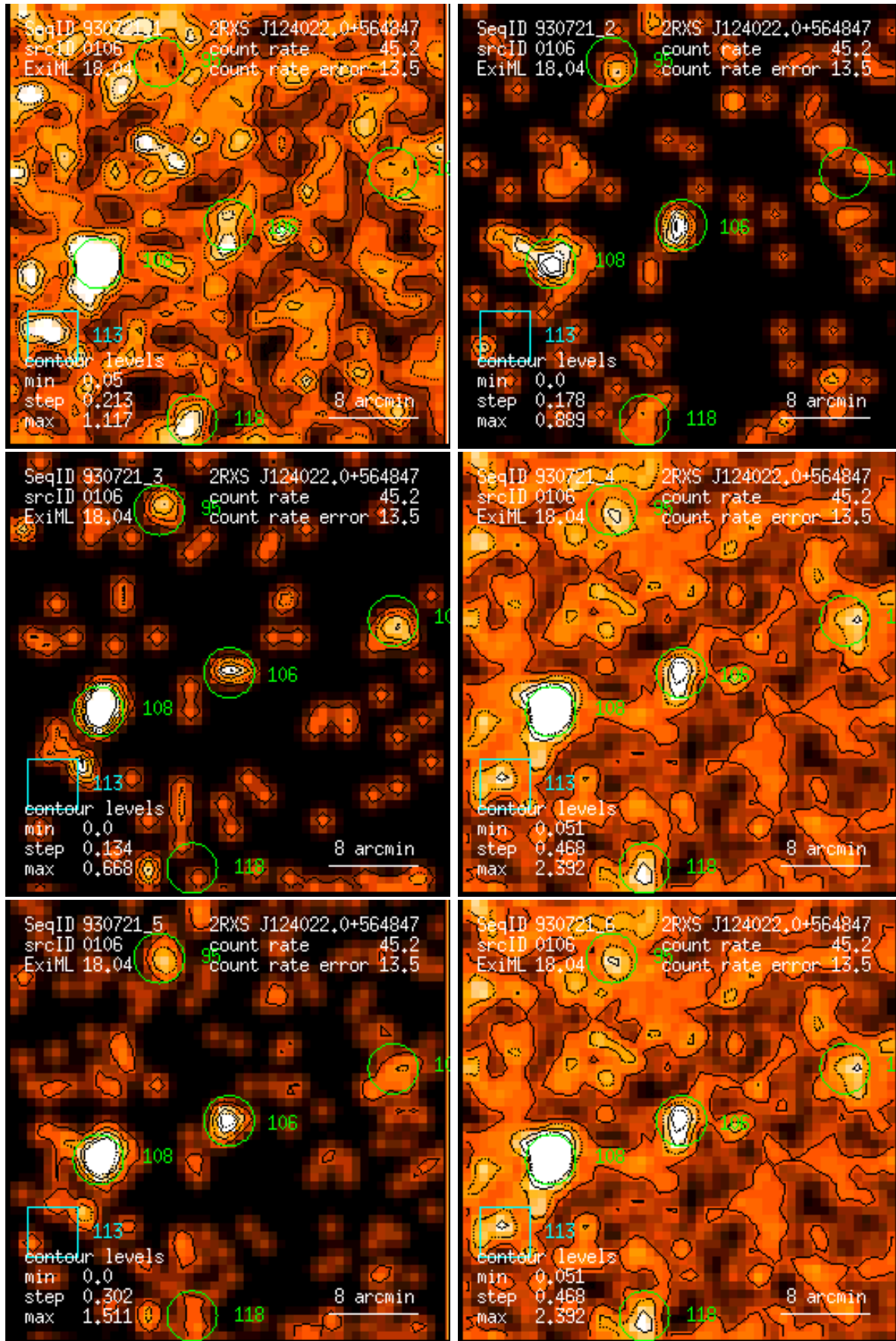
Figure 106: RASS 930721: detection 0106: band rate images, Gaussian filter: (1) PSPC channels 11 – 41, (2) 52 – 90, (3) 91 – 201, (4) 11 – 235, (5) 52 – 201, (6) 11 – 201. Broad band rates in counts/ks. Band rate contour levels in counts/ks/arcmin 2 .
