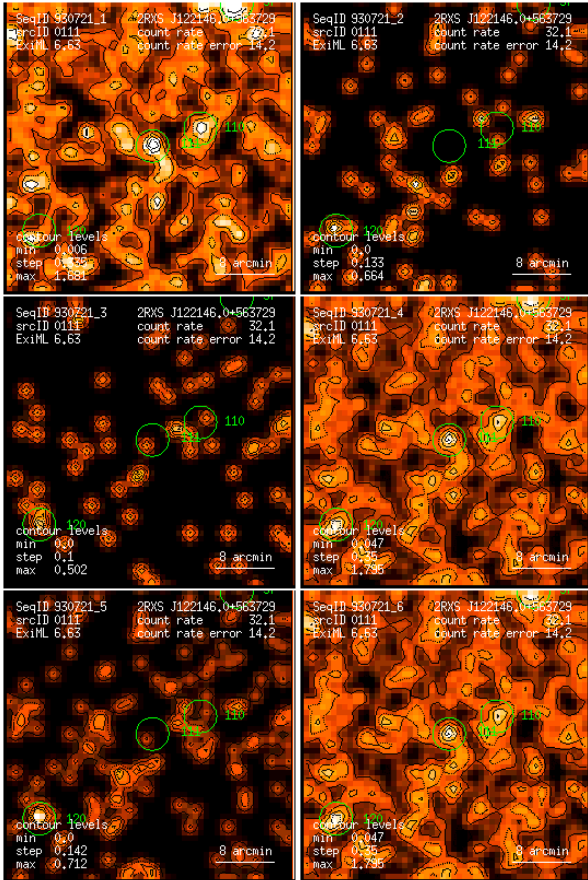
Figure 111: RASS 930721: detection 0111: band rate images, Gaussian filter: (1) PSPC channels 11 – 41, (2) 52 – 90, (3) 91 – 201, (4) 11 – 235, (5) 52 – 201, (6) 11 – 201. Broad band rates in counts/ks. Band rate contour levels in counts/ks/arcmin 2 .
