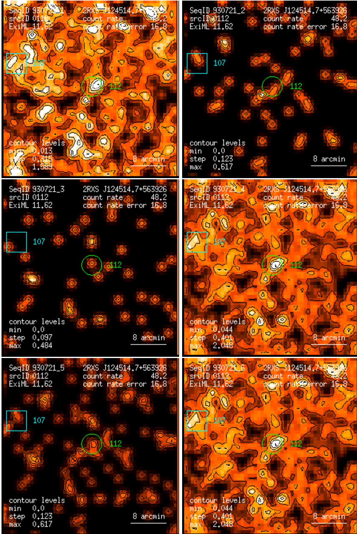
Figure 112: RASS 930721: detection 0112: band rate images, Gaussian filter: (1) PSPC channels 11 – 41, (2) 52 – 90, (3) 91 – 201, (4) 11 – 235, (5) 52 – 201, (6) 11 – 201. Broad band rates in counts/ks. Band rate contour levels in counts/ks/arcmin 2 .
