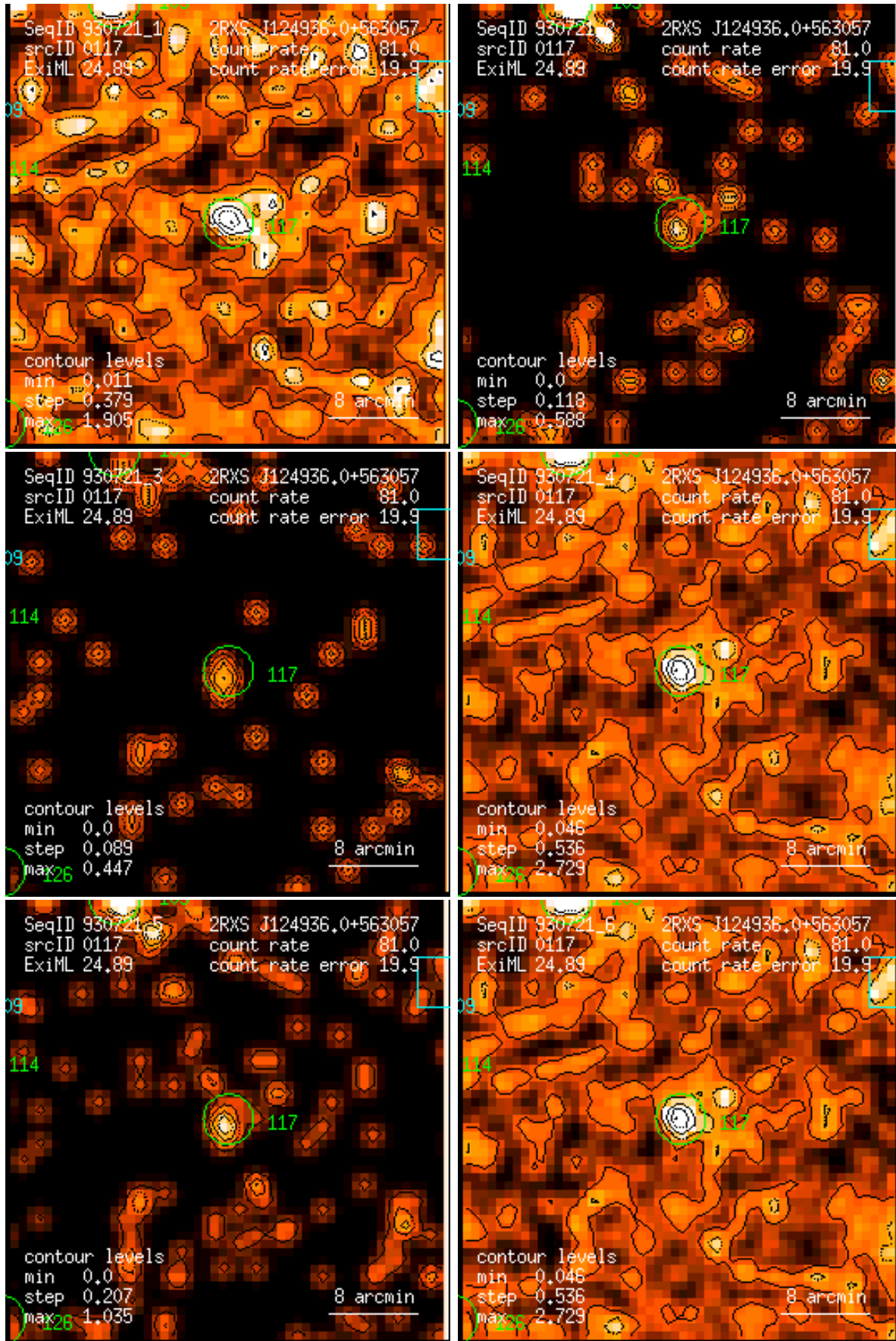
Figure 117: RASS 930721: detection 0117: band rate images, Gaussian filter: (1) PSPC channels 11 – 41, (2) 52 – 90, (3) 91 – 201, (4) 11 – 235, (5) 52 – 201, (6) 11 – 201. Broad band rates in counts/ks. Band rate contour levels in counts/ks/arcmin 2 .
