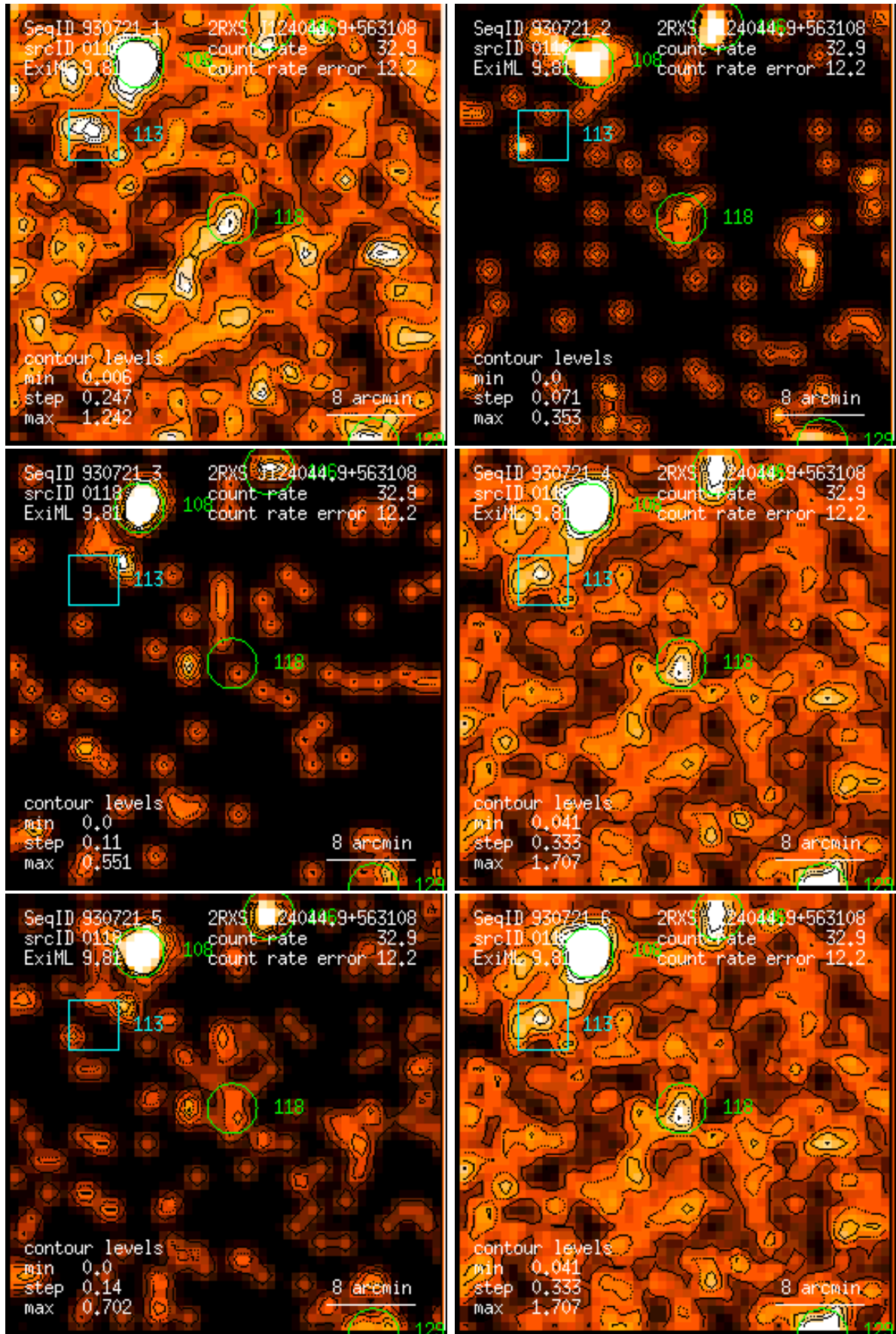
Figure 118: RASS 930721: detection 0118: band rate images, Gaussian filter: (1) PSPC channels 11 – 41, (2) 52 – 90, (3) 91 – 201, (4) 11 – 235, (5) 52 – 201, (6) 11 – 201. Broad band rates in counts/ks. Band rate contour levels in counts/ks/arcmin 2 .
