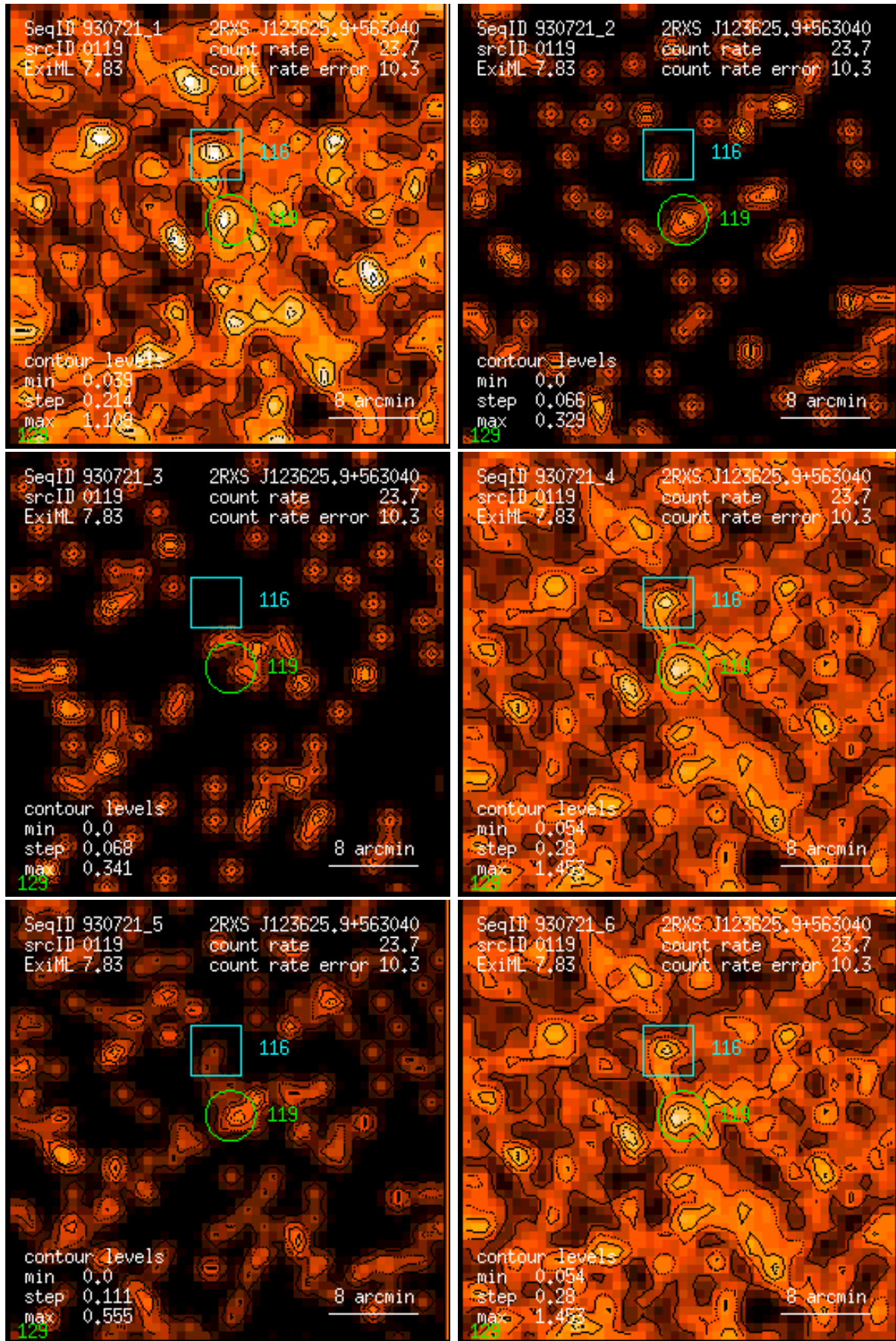
Figure 119: RASS 930721: detection 0119: band rate images, Gaussian filter: (1) PSPC channels 11 – 41, (2) 52 – 90, (3) 91 – 201, (4) 11 – 235, (5) 52 – 201, (6) 11 – 201. Broad band rates in counts/ks. Band rate contour levels in counts/ks/arcmin 2 .
