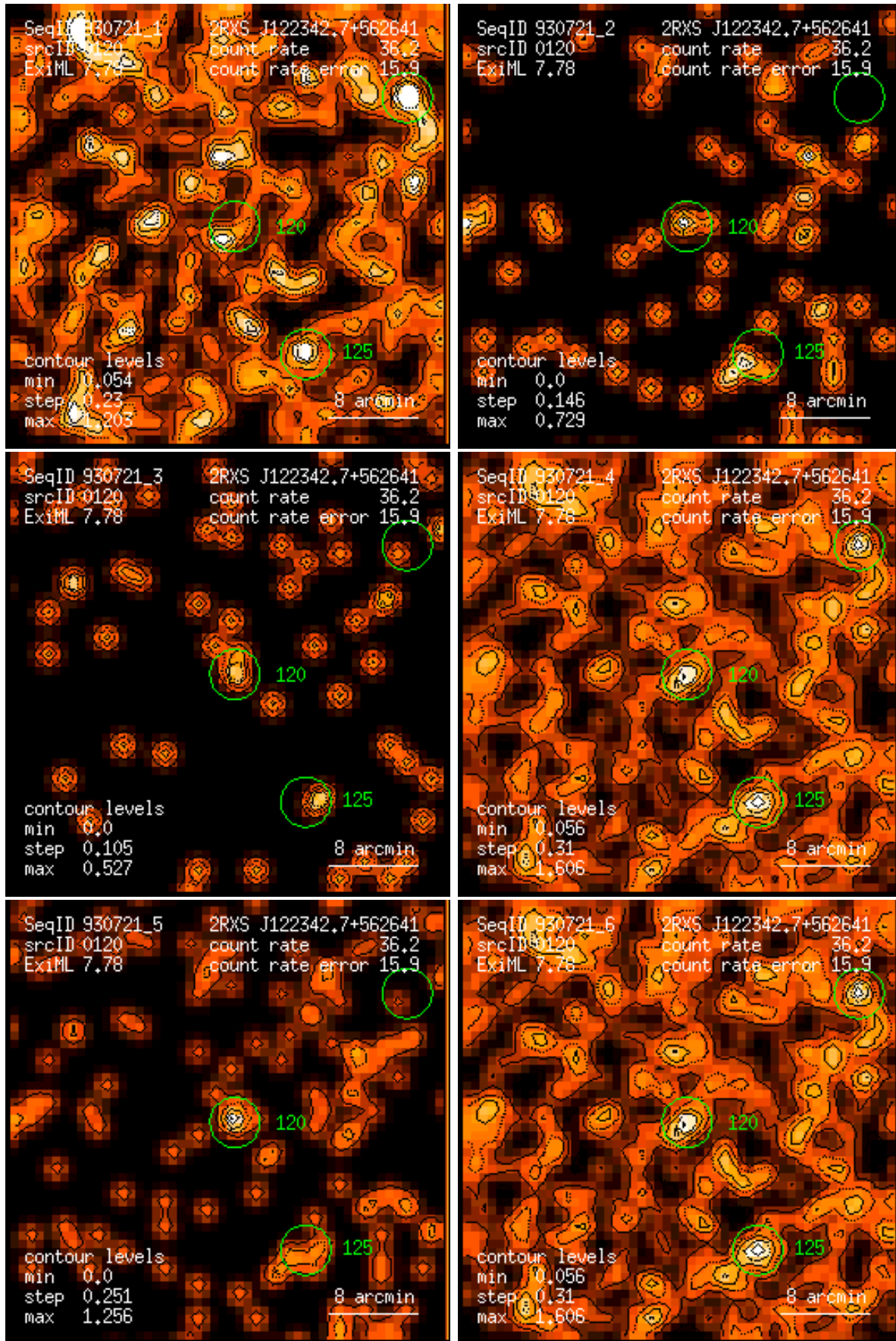
Figure 120: RASS 930721: detection 0120: band rate images, Gaussian filter: (1) PSPC channels 11 – 41, (2) 52 – 90, (3) 91 – 201, (4) 11 – 235, (5) 52 – 201, (6) 11 – 201. Broad band rates in counts/ks. Band rate contour levels in counts/ks/arcmin 2 .
