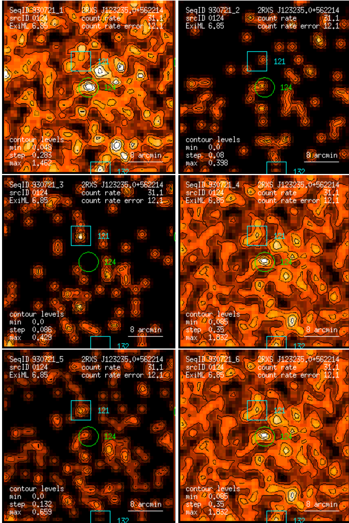
Figure 124: RASS 930721: detection 0124: band rate images, Gaussian filter: (1) PSPC channels 11 – 41, (2) 52 – 90, (3) 91 – 201, (4) 11 – 235, (5) 52 – 201, (6) 11 – 201. Broad band rates in counts/ks. Band rate contour levels in counts/ks/arcmin 2 .
