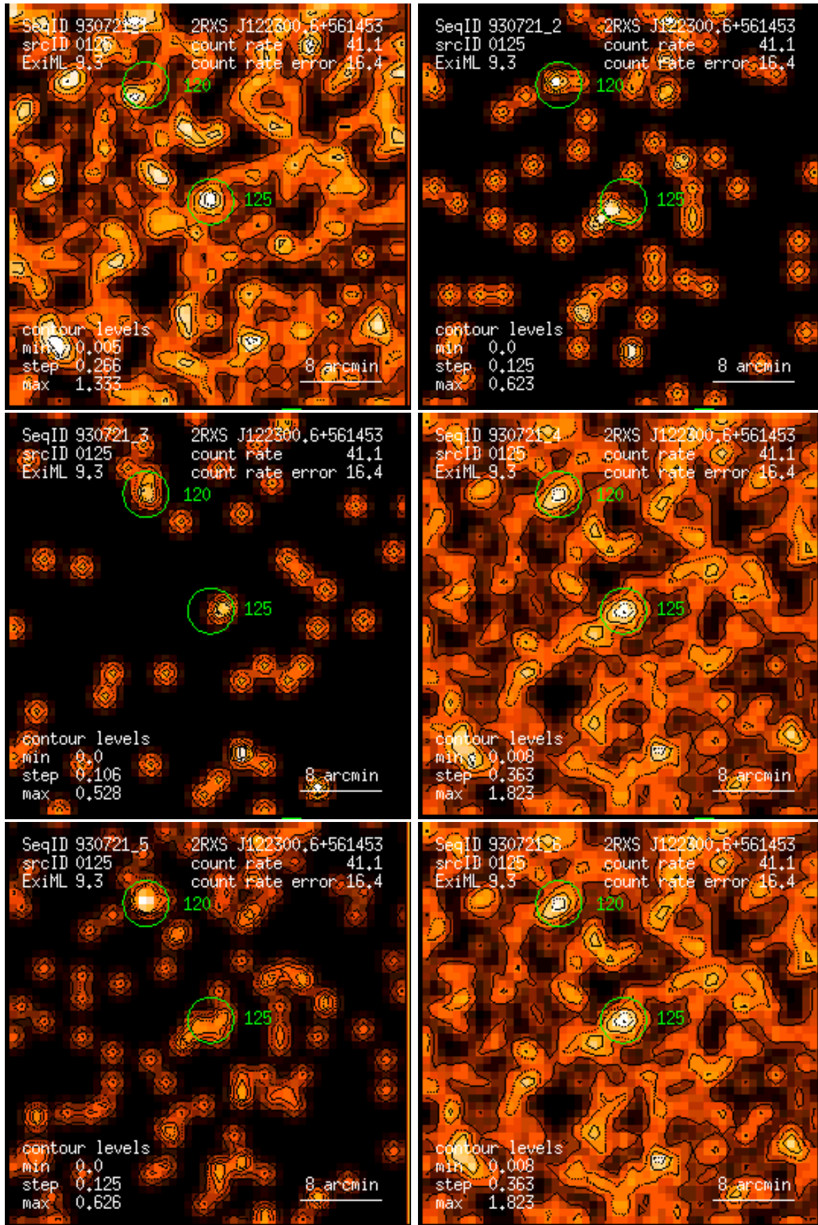
Figure 125: RASS 930721: detection 0125: band rate images, Gaussian filter: (1) PSPC channels 11 – 41, (2) 52 – 90, (3) 91 – 201, (4) 11 – 235, (5) 52 – 201, (6) 11 – 201. Broad band rates in counts/ks. Band rate contour levels in counts/ks/arcmin 2 .
