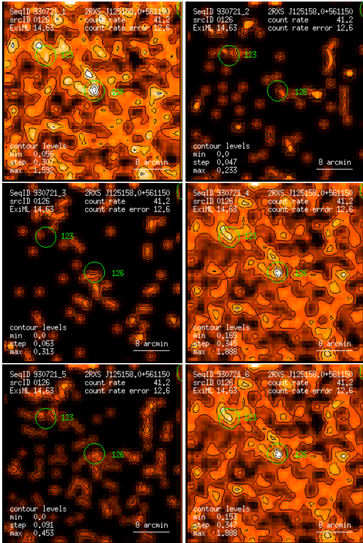
Figure 126: RASS 930721: detection 0126: band rate images, Gaussian filter: (1) PSPC channels 11 – 41, (2) 52 – 90, (3) 91 – 201, (4) 11 – 235, (5) 52 – 201, (6) 11 – 201. Broad band rates in counts/ks. Band rate contour levels in counts/ks/arcmin 2 .
