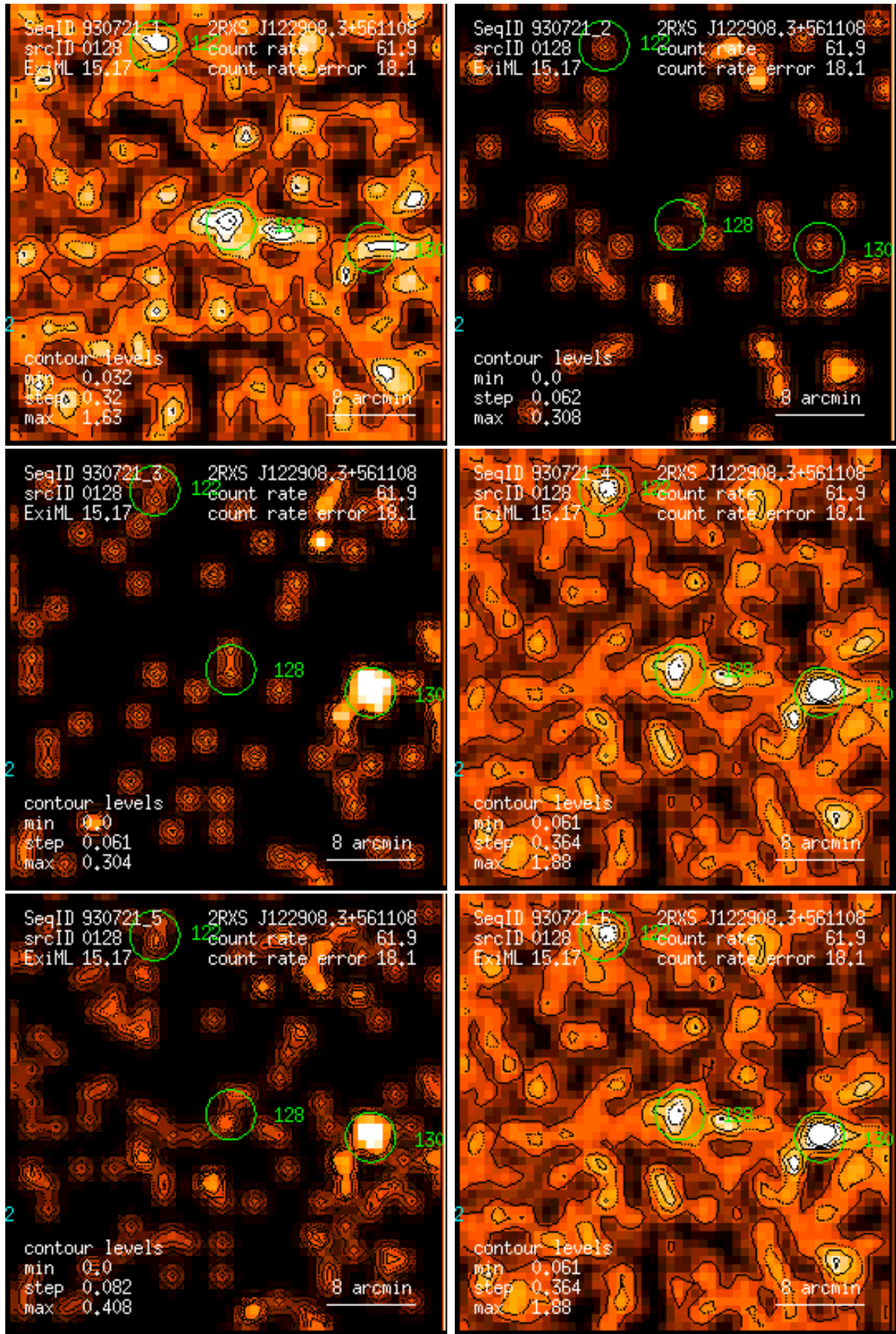
Figure 128: RASS 930721: detection 0128: band rate images, Gaussian filter: (1) PSPC channels 11 – 41, (2) 52 – 90, (3) 91 – 201, (4) 11 – 235, (5) 52 – 201, (6) 11 – 201. Broad band rates in counts/ks. Band rate contour levels in counts/ks/arcmin 2 .
