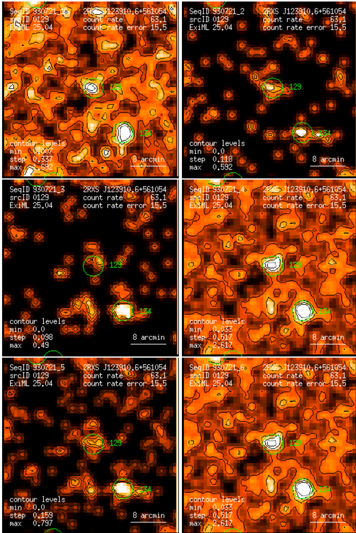
Figure 129: RASS 930721: detection 0129: band rate images, Gaussian filter: (1) PSPC channels 11 – 41, (2) 52 – 90, (3) 91 – 201, (4) 11 – 235, (5) 52 – 201, (6) 11 – 201. Broad band rates in counts/ks. Band rate contour levels in counts/ks/arcmin 2 .
