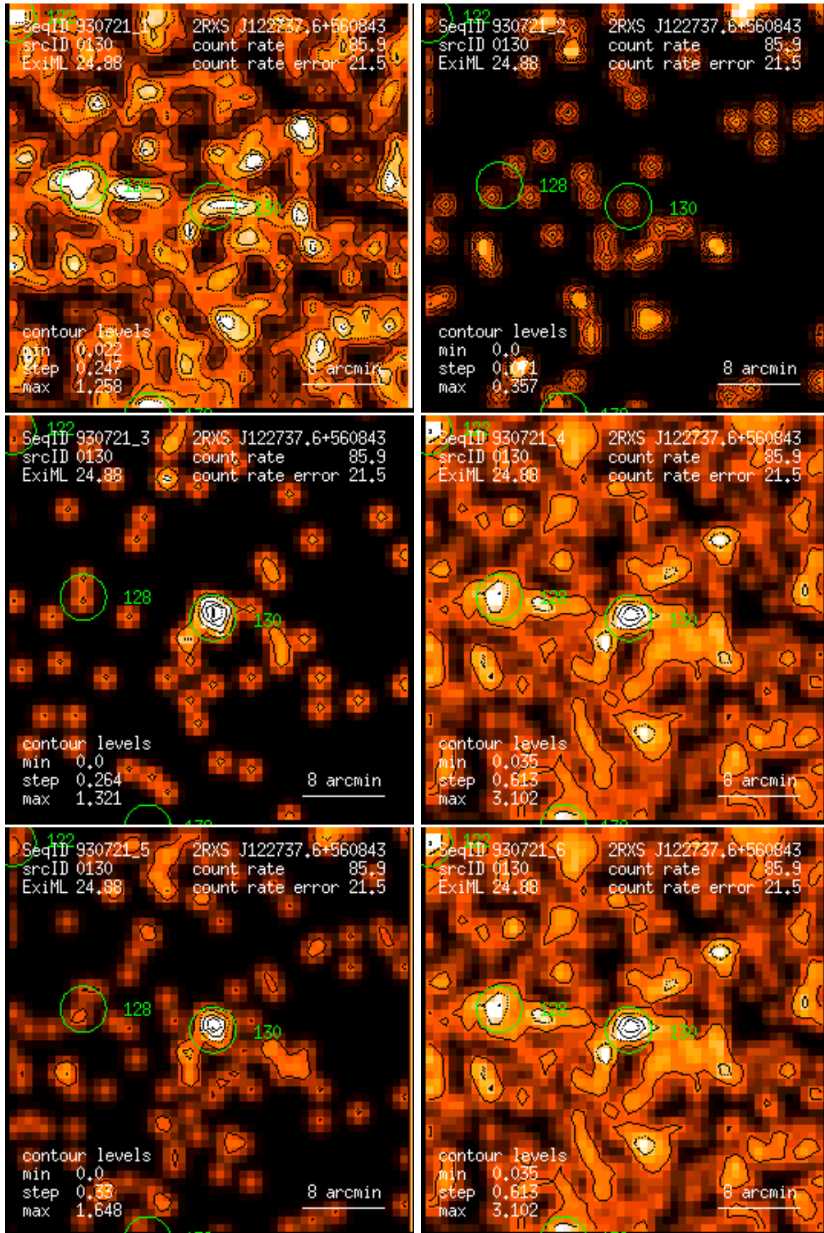
Figure 130: RASS 930721: detection 0130: band rate images, Gaussian filter: (1) PSPC channels 11 – 41, (2) 52 – 90, (3) 91 – 201, (4) 11 – 235, (5) 52 – 201, (6) 11 – 201. Broad band rates in counts/ks. Band rate contour levels in counts/ks/arcmin 2 .
