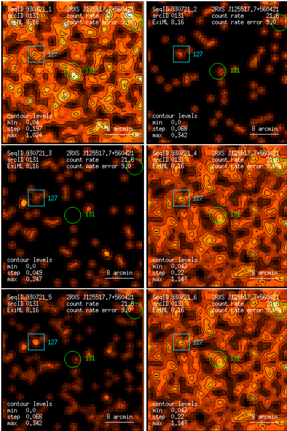
Figure 131: RASS 930721: detection 0131: band rate images, Gaussian filter: (1) PSPC channels 11 – 41, (2) 52 – 90, (3) 91 – 201, (4) 11 – 235, (5) 52 – 201, (6) 11 – 201. Broad band rates in counts/ks. Band rate contour levels in counts/ks/arcmin 2 .
