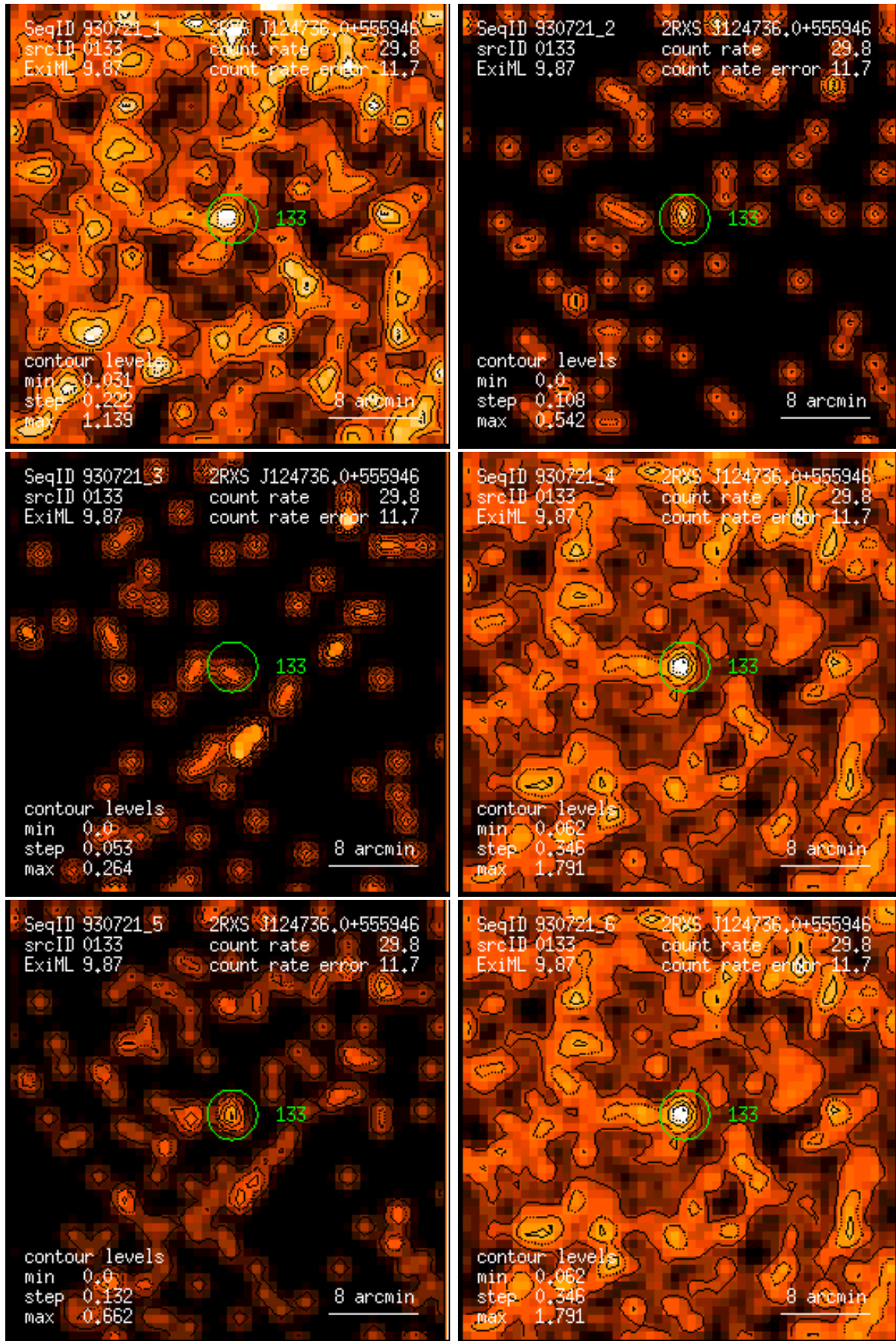
Figure 133: RASS 930721: detection 0133: band rate images, Gaussian filter: (1) PSPC channels 11 – 41, (2) 52 – 90, (3) 91 – 201, (4) 11 – 235, (5) 52 – 201, (6) 11 – 201. Broad band rates in counts/ks. Band rate contour levels in counts/ks/arcmin 2 .
