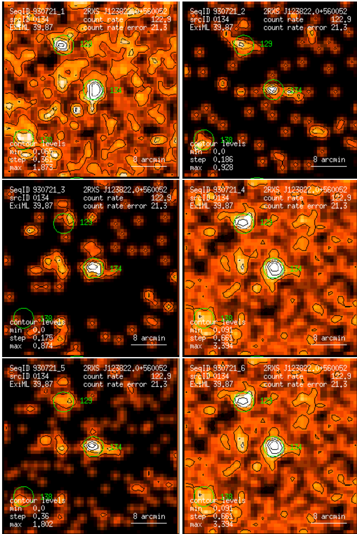
Figure 134: RASS 930721: detection 0134: band rate images, Gaussian filter: (1) PSPC channels 11 – 41, (2) 52 – 90, (3) 91 – 201, (4) 11 – 235, (5) 52 – 201, (6) 11 – 201. Broad band rates in counts/ks. Band rate contour levels in counts/ks/arcmin 2 .
