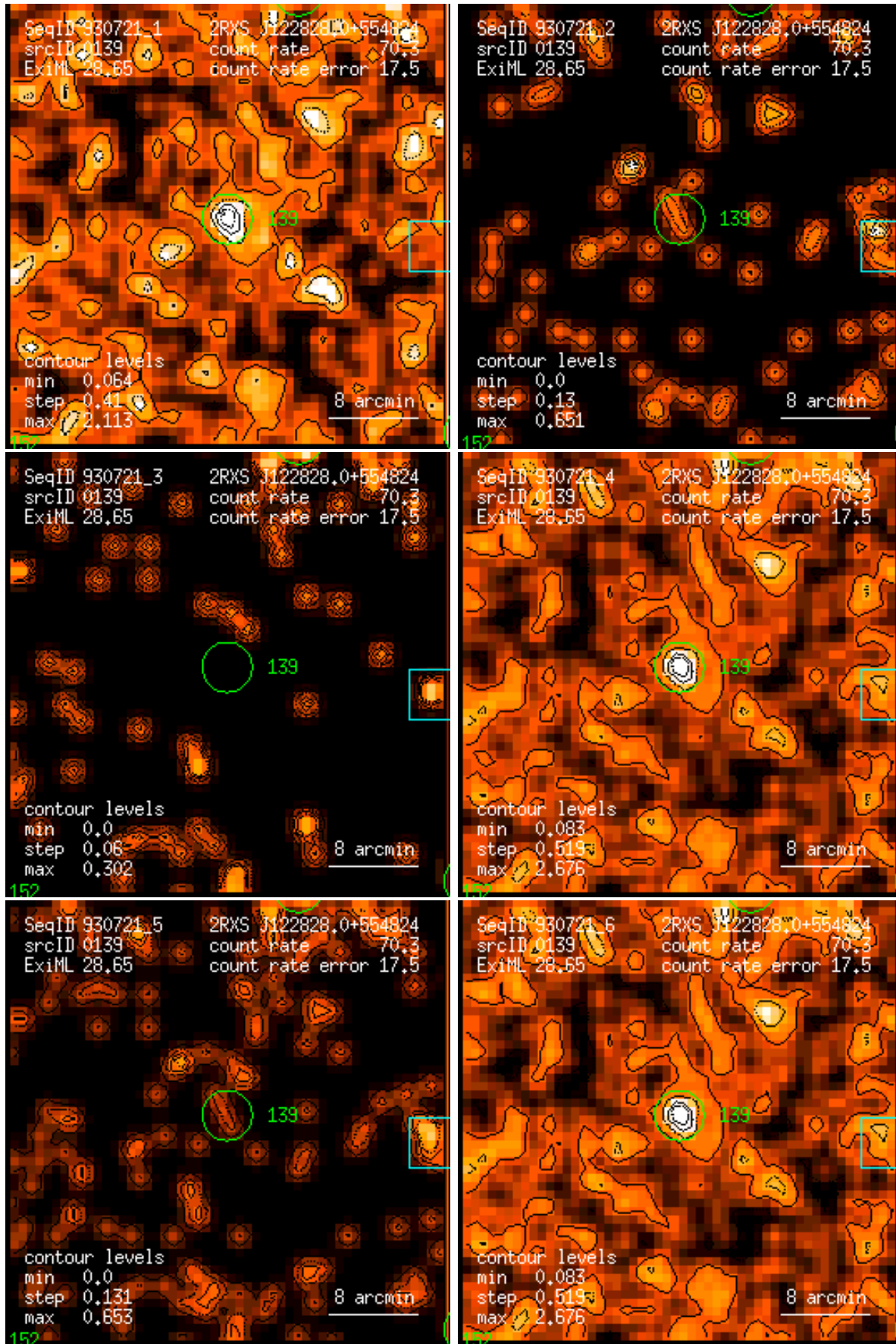
Figure 139: RASS 930721: detection 0139: band rate images, Gaussian filter: (1) PSPC channels 11 – 41, (2) 52 – 90, (3) 91 – 201, (4) 11 – 235, (5) 52 – 201, (6) 11 – 201. Broad band rates in counts/ks. Band rate contour levels in counts/ks/arcmin 2 .
