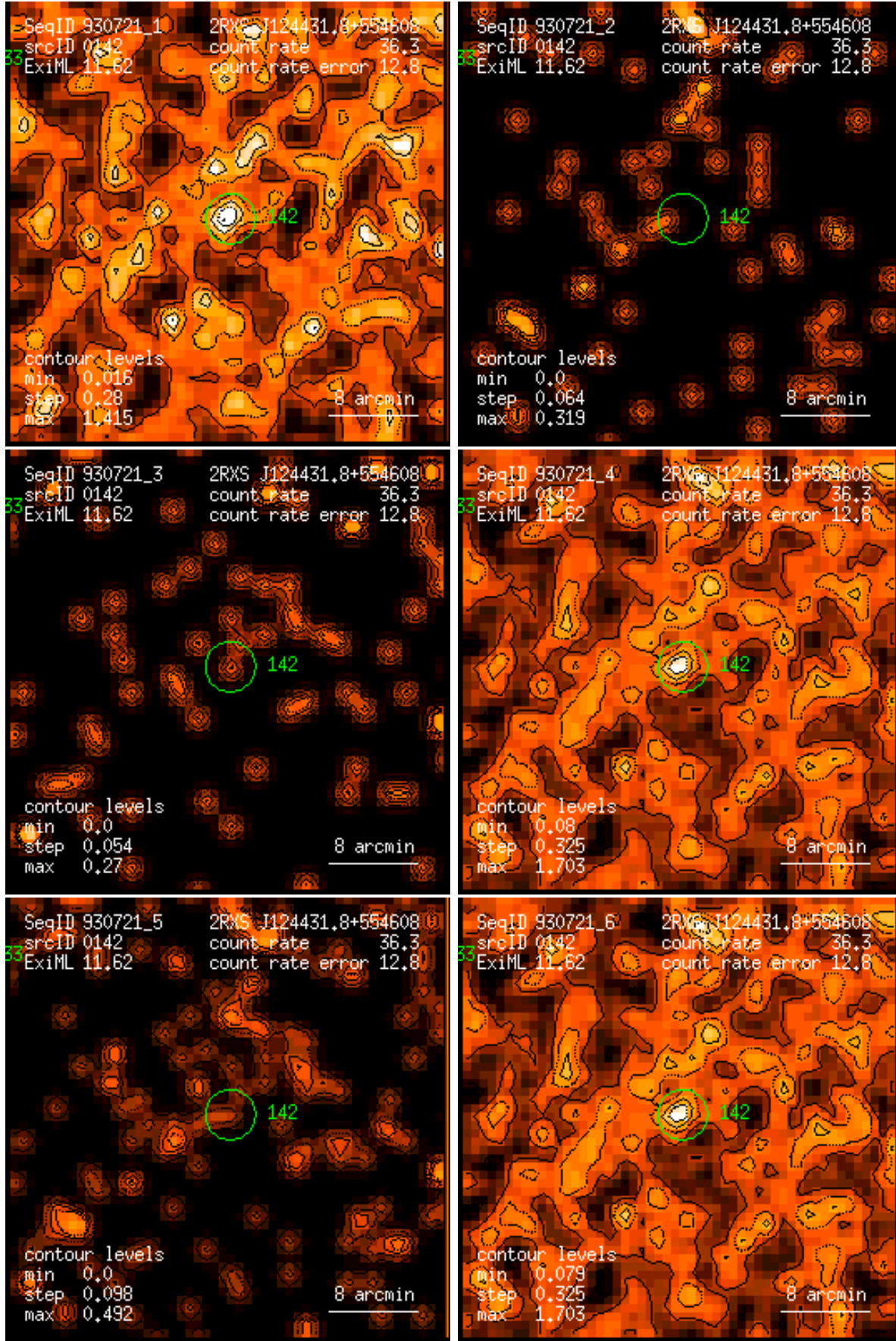
Figure 142: RASS 930721: detection 0142: band rate images, Gaussian filter: (1) PSPC channels 11 – 41, (2) 52 – 90, (3) 91 – 201, (4) 11 – 235, (5) 52 – 201, (6) 11 – 201. Broad band rates in counts/ks. Band rate contour levels in counts/ks/arcmin 2 .
