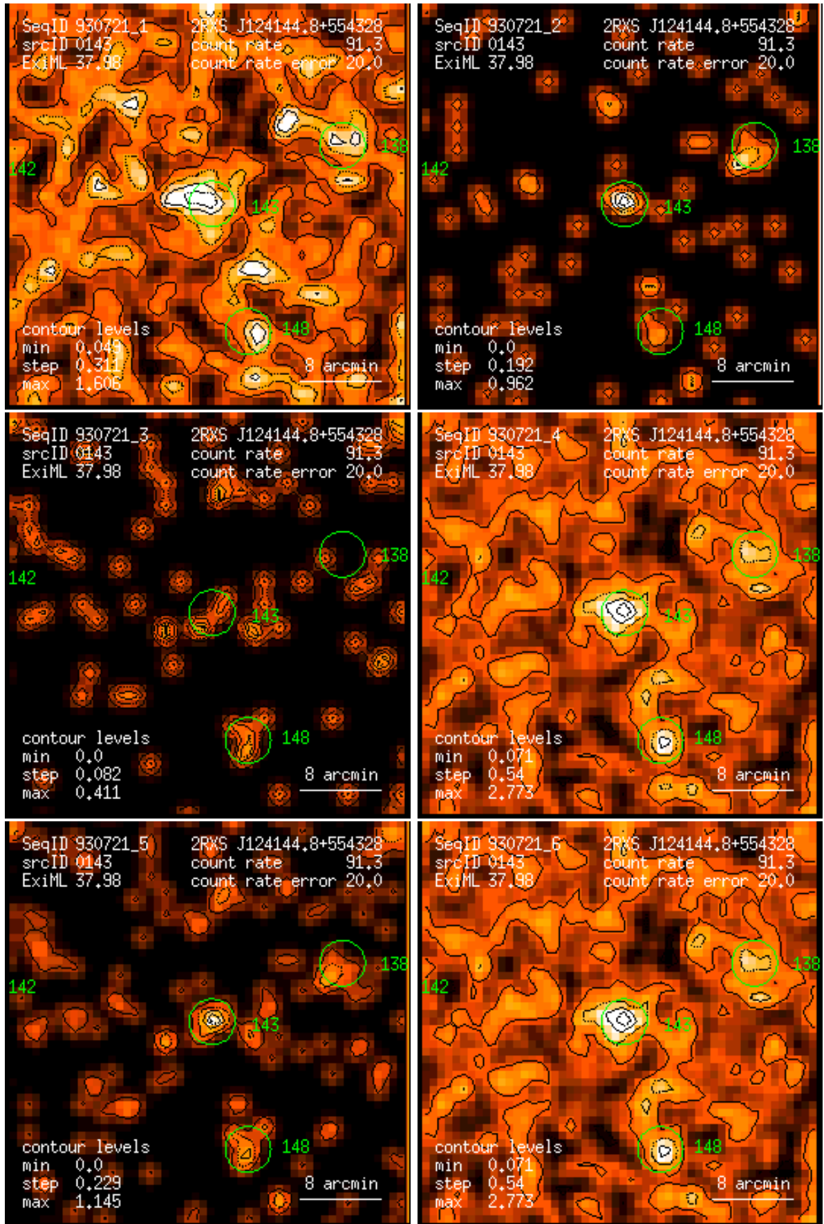
Figure 143: RASS 930721: detection 0143: band rate images, Gaussian filter: (1) PSPC channels 11 – 41, (2) 52 – 90, (3) 91 – 201, (4) 11 – 235, (5) 52 – 201, (6) 11 – 201. Broad band rates in counts/ks. Band rate contour levels in counts/ks/arcmin 2 .
