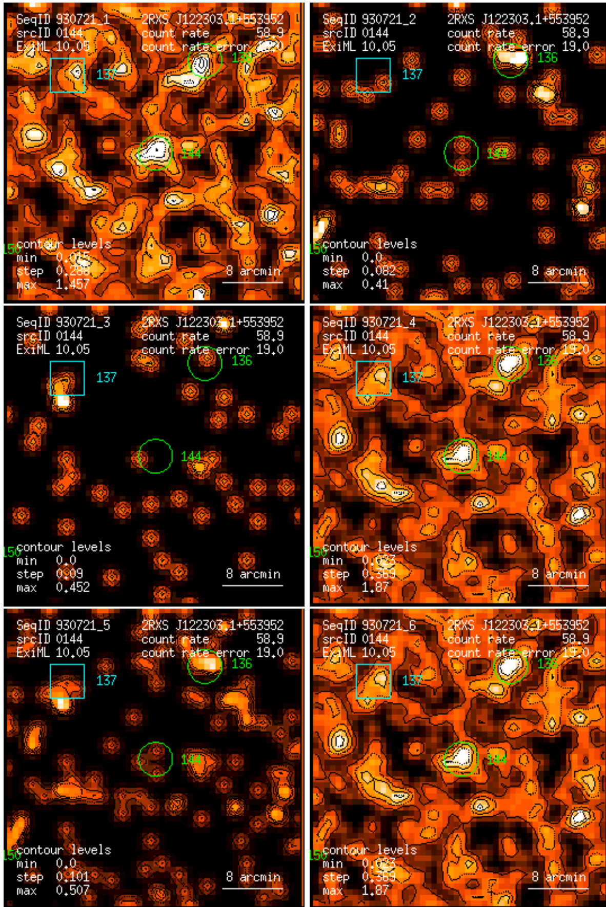
Figure 144: RASS 930721: detection 0144: band rate images, Gaussian filter: (1) PSPC channels 11 – 41, (2) 52 – 90, (3) 91 – 201, (4) 11 – 235, (5) 52 – 201, (6) 11 – 201. Broad band rates in counts/ks. Band rate contour levels in counts/ks/arcmin 2 .
