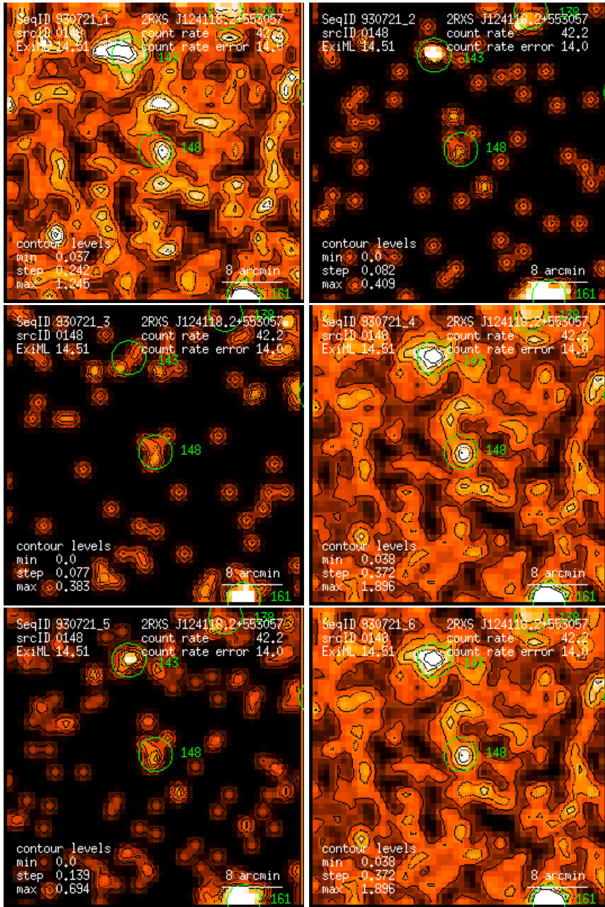
Figure 148: RASS 930721: detection 0148: band rate images, Gaussian filter: (1) PSPC channels 11 – 41, (2) 52 – 90, (3) 91 – 201, (4) 11 – 235, (5) 52 – 201, (6) 11 – 201. Broad band rates in counts/ks. Band rate contour levels in counts/ks/arcmin 2 .
