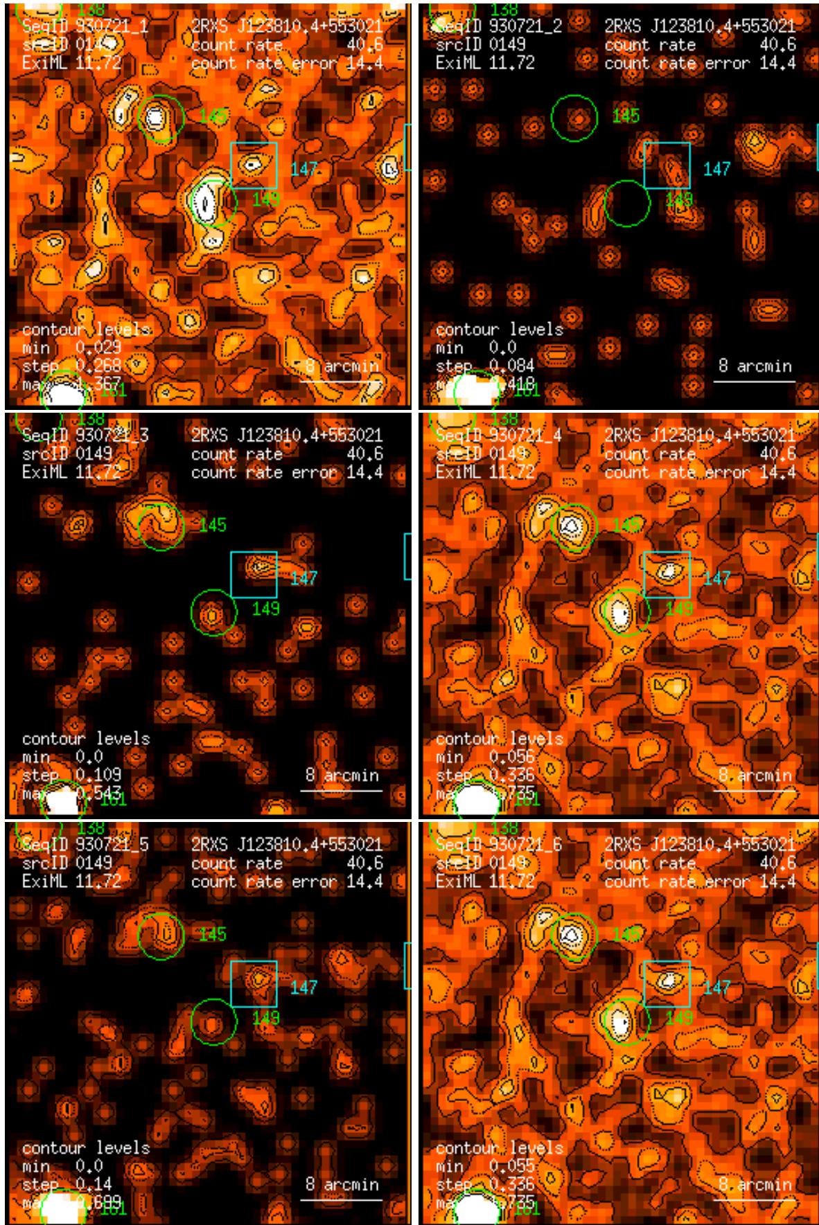
Figure 149: RASS 930721: detection 0149: band rate images, Gaussian filter: (1) PSPC channels 11 – 41, (2) 52 – 90, (3) 91 – 201, (4) 11 – 235, (5) 52 – 201, (6) 11 – 201. Broad band rates in counts/ks. Band rate contour levels in counts/ks/arcmin 2 .
