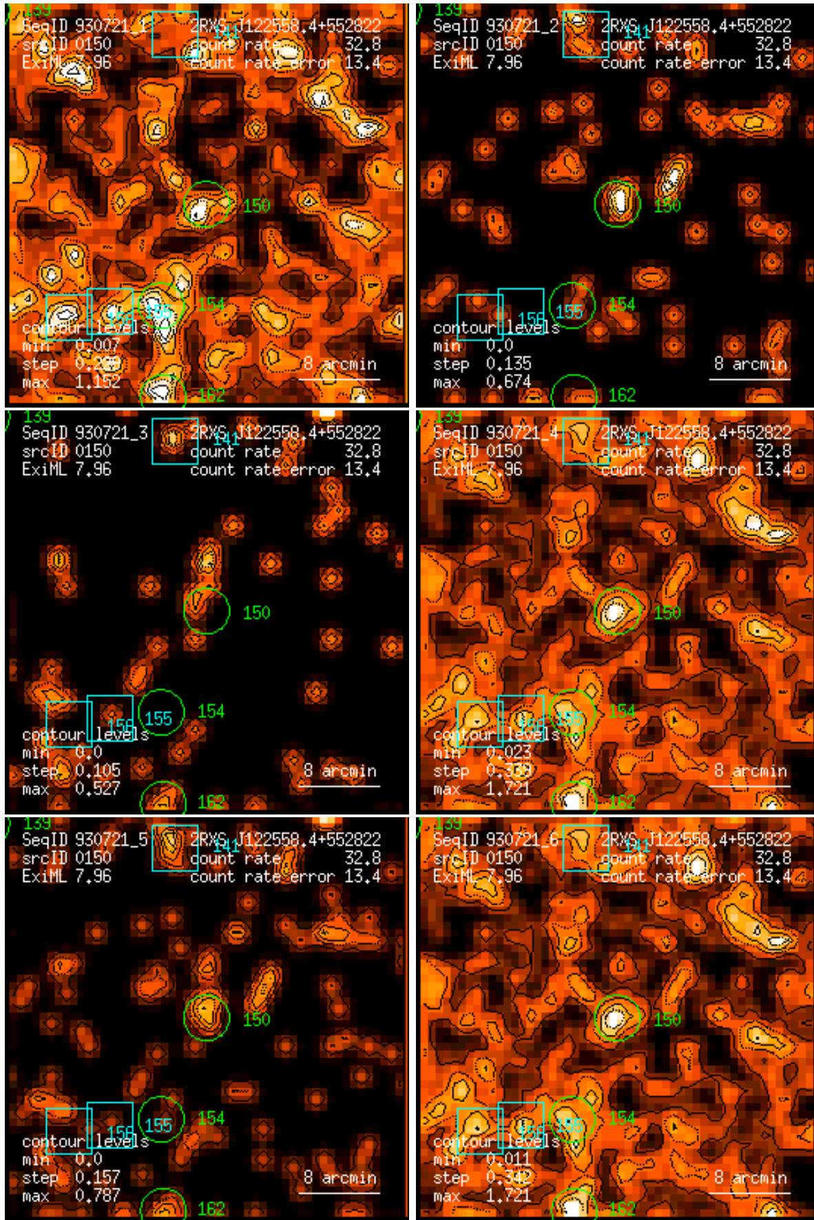
Figure 150: RASS 930721: detection 0150: band rate images, Gaussian filter: (1) PSPC channels 11 – 41, (2) 52 – 90, (3) 91 – 201, (4) 11 – 235, (5) 52 – 201, (6) 11 – 201. Broad band rates in counts/ks. Band rate contour levels in counts/ks/arcmin 2 .
