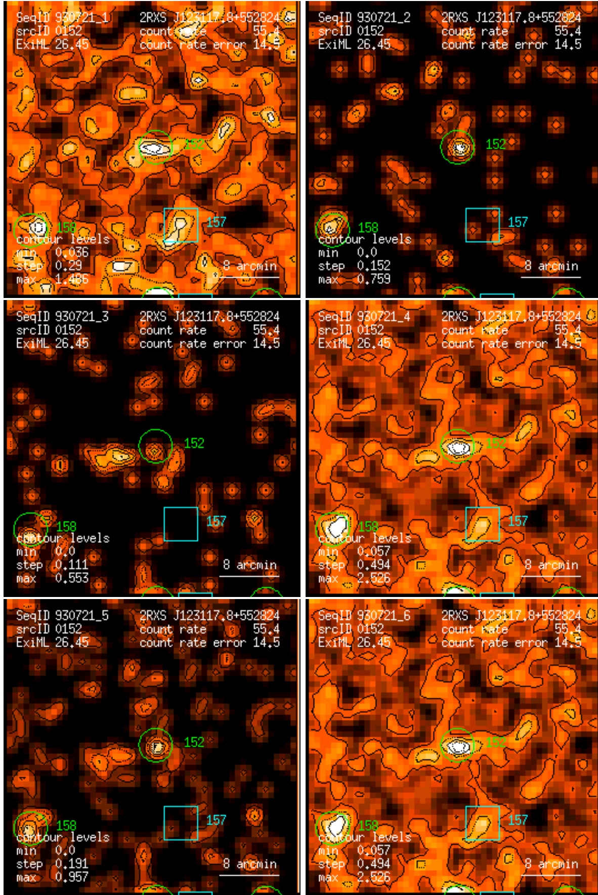
Figure 152: RASS 930721: detection 0152: band rate images, Gaussian filter: (1) PSPC channels 11 – 41, (2) 52 – 90, (3) 91 – 201, (4) 11 – 235, (5) 52 – 201, (6) 11 – 201. Broad band rates in counts/ks. Band rate contour levels in counts/ks/arcmin 2 .
