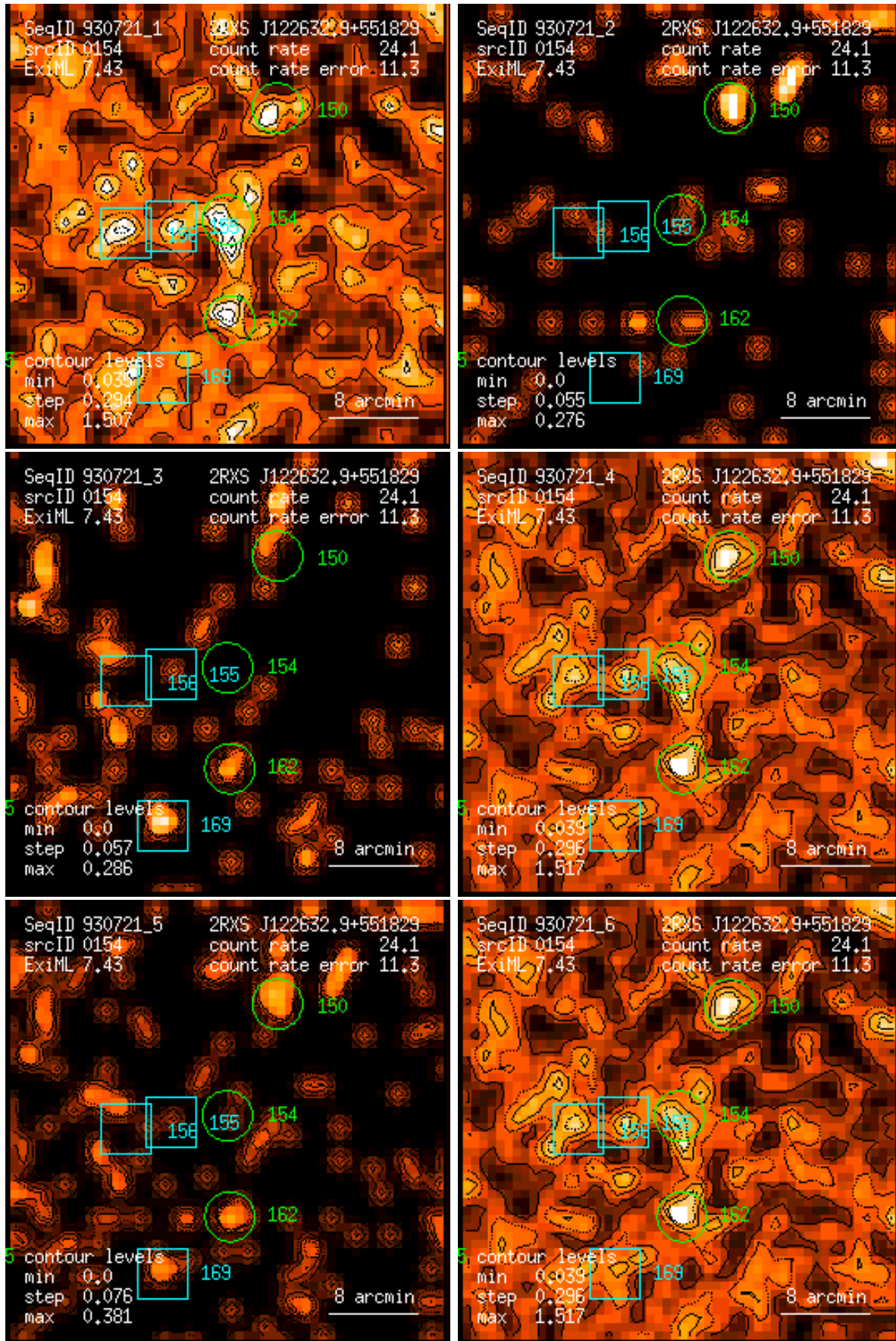
Figure 154: RASS 930721: detection 0154: band rate images, Gaussian filter: (1) PSPC channels 11 – 41, (2) 52 – 90, (3) 91 – 201, (4) 11 – 235, (5) 52 – 201, (6) 11 – 201. Broad band rates in counts/ks. Band rate contour levels in counts/ks/arcmin 2 .
