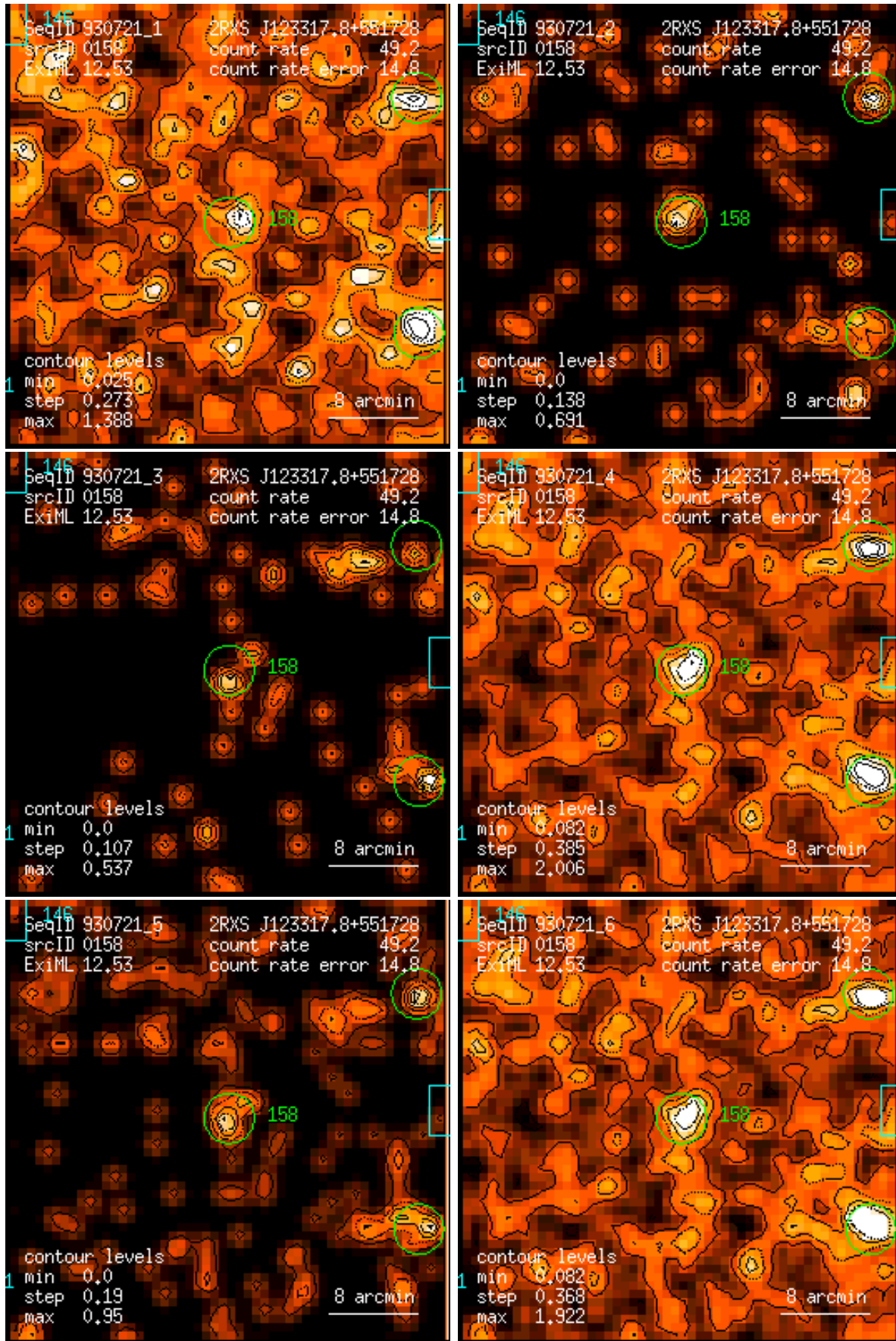
Figure 158: RASS 930721: detection 0158: band rate images, Gaussian filter: (1) PSPC channels 11 – 41, (2) 52 – 90, (3) 91 – 201, (4) 11 – 235, (5) 52 – 201, (6) 11 – 201. Broad band rates in counts/ks. Band rate contour levels in counts/ks/arcmin 2 .
