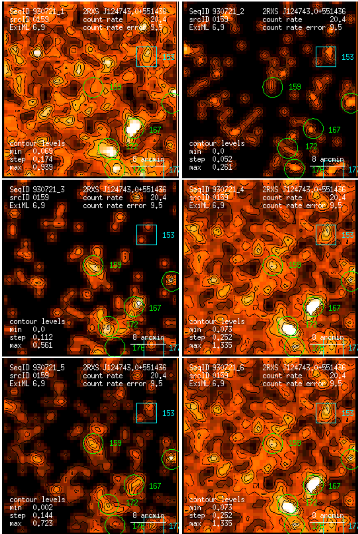
Figure 159: RASS 930721: detection 0159: band rate images, Gaussian filter: (1) PSPC channels 11 – 41, (2) 52 – 90, (3) 91 – 201, (4) 11 – 235, (5) 52 – 201, (6) 11 – 201. Broad band rates in counts/ks. Band rate contour levels in counts/ks/arcmin 2 .
