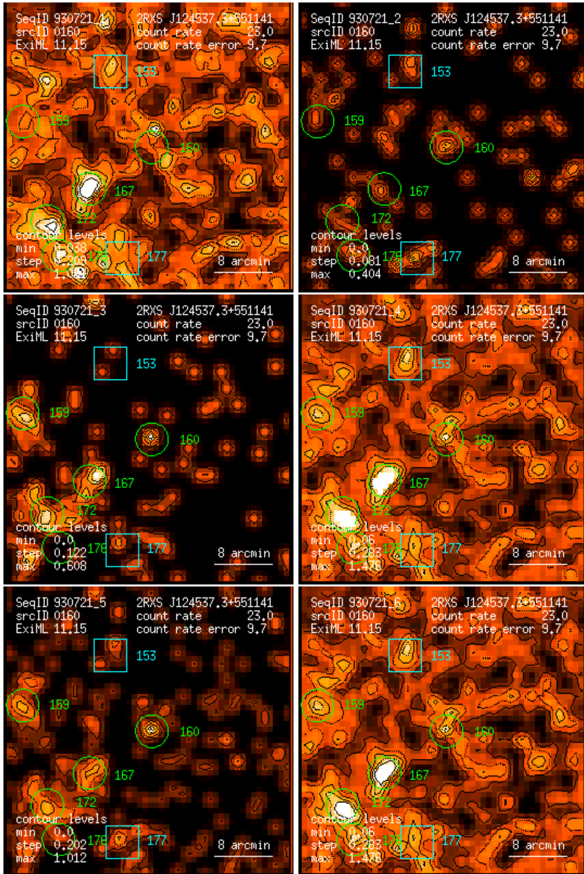
Figure 160: RASS 930721: detection 0160: band rate images, Gaussian filter: (1) PSPC channels 11 – 41, (2) 52 – 90, (3) 91 – 201, (4) 11 – 235, (5) 52 – 201, (6) 11 – 201. Broad band rates in counts/ks. Band rate contour levels in counts/ks/arcmin 2 .
