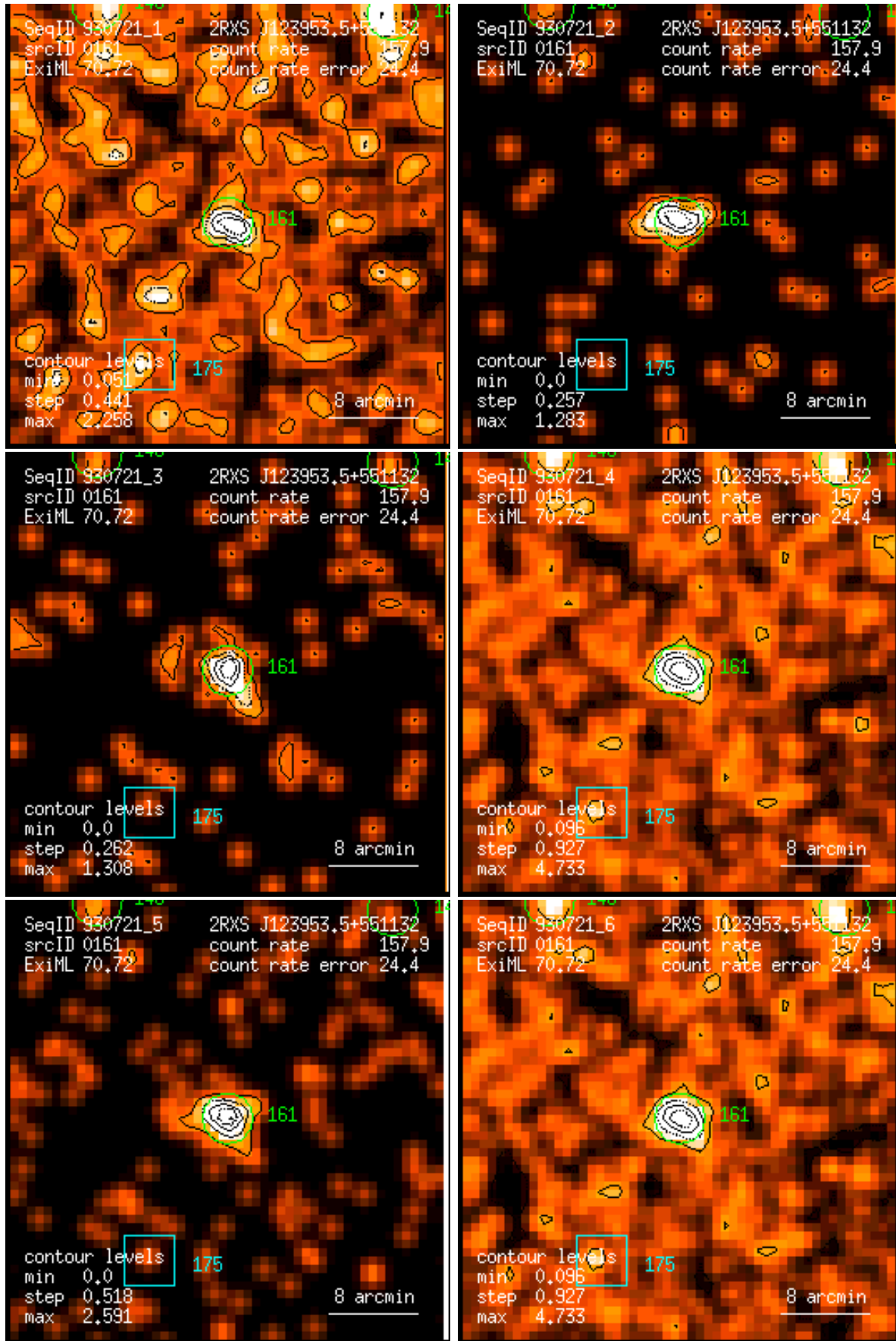
Figure 161: RASS 930721: detection 0161: band rate images, Gaussian filter: (1) PSPC channels 11 – 41, (2) 52 – 90, (3) 91 – 201, (4) 11 – 235, (5) 52 – 201, (6) 11 – 201. Broad band rates in counts/ks. Band rate contour levels in counts/ks/arcmin 2 .
