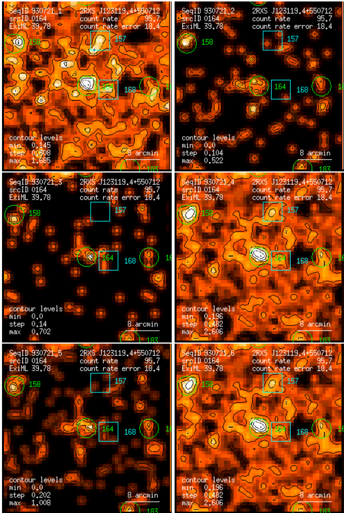
Figure 164: RASS 930721: detection 0164: band rate images, Gaussian filter: (1) PSPC channels 11 – 41, (2) 52 – 90, (3) 91 – 201, (4) 11 – 235, (5) 52 – 201, (6) 11 – 201. Broad band rates in counts/ks. Band rate contour levels in counts/ks/arcmin 2 .
