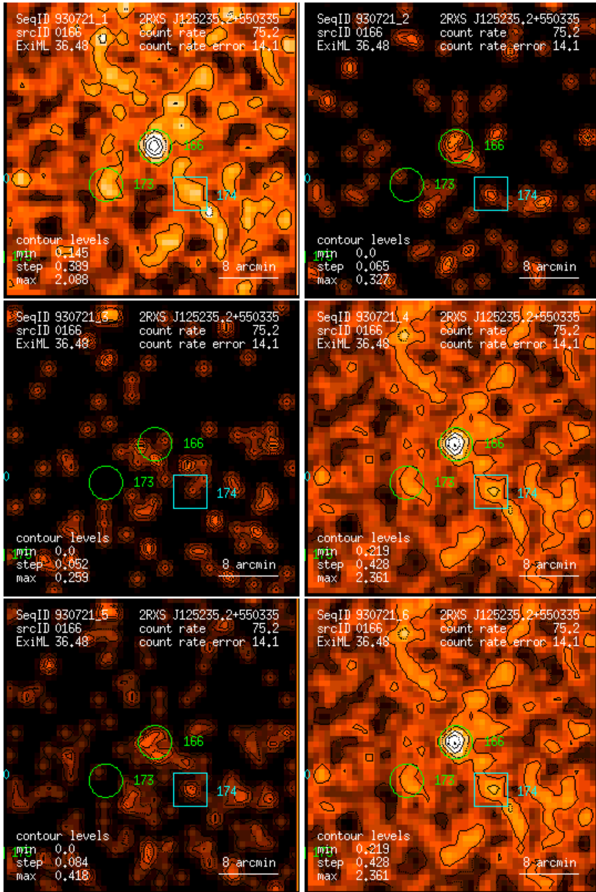
Figure 166: RASS 930721: detection 0166: band rate images, Gaussian filter: (1) PSPC channels 11 – 41, (2) 52 – 90, (3) 91 – 201, (4) 11 – 235, (5) 52 – 201, (6) 11 – 201. Broad band rates in counts/ks. Band rate contour levels in counts/ks/arcmin 2 .
