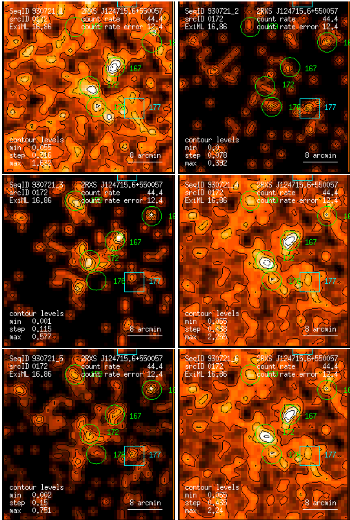
Figure 172: RASS 930721: detection 0172: band rate images, Gaussian filter: (1) PSPC channels 11 – 41, (2) 52 – 90, (3) 91 – 201, (4) 11 – 235, (5) 52 – 201, (6) 11 – 201. Broad band rates in counts/ks. Band rate contour levels in counts/ks/arcmin 2 .
