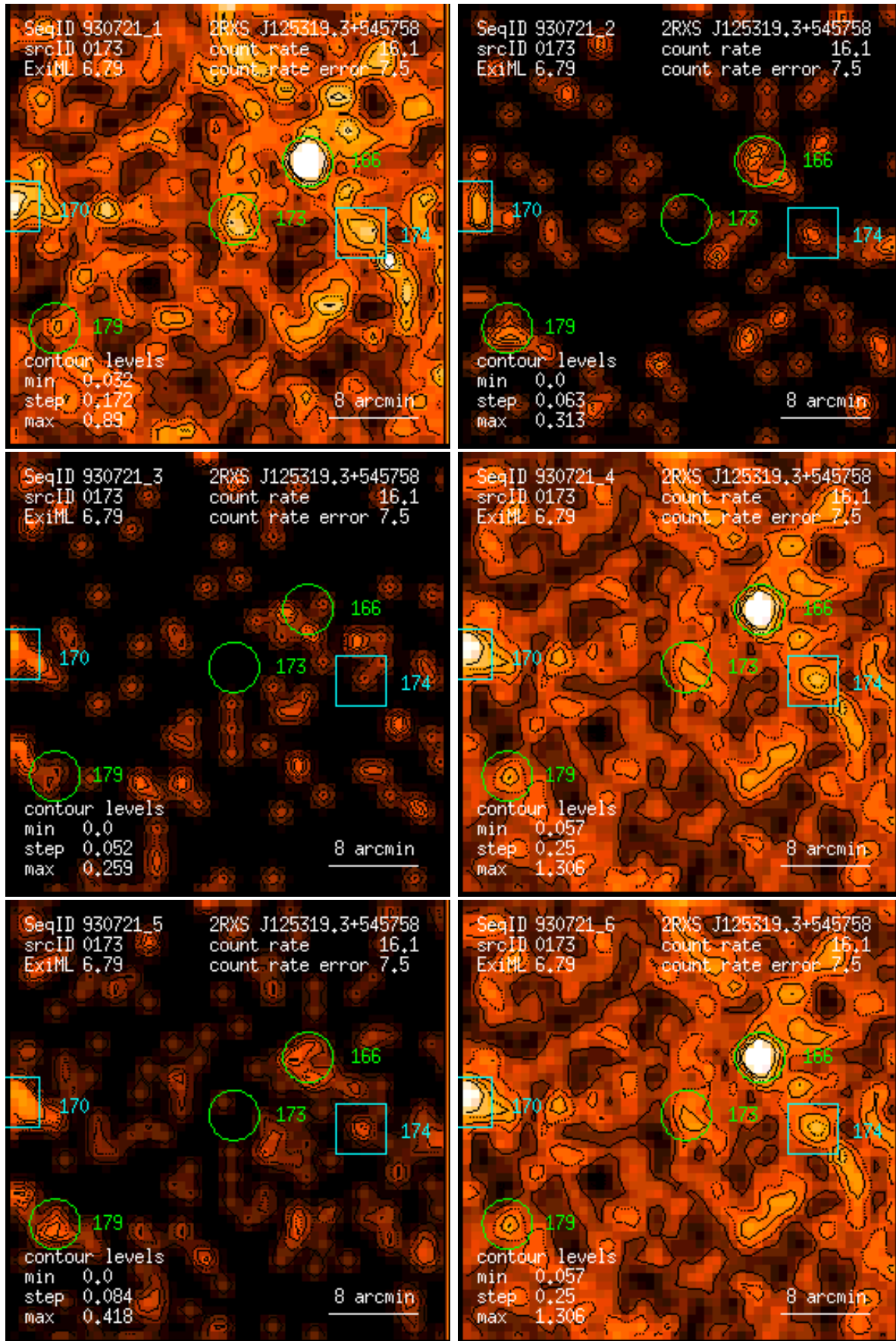
Figure 173: RASS 930721: detection 0173: band rate images, Gaussian filter: (1) PSPC channels 11 – 41, (2) 52 – 90, (3) 91 – 201, (4) 11 – 235, (5) 52 – 201, (6) 11 – 201. Broad band rates in counts/ks. Band rate contour levels in counts/ks/arcmin 2 .
