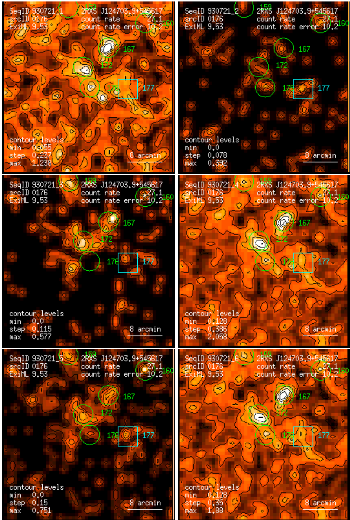
Figure 176: RASS 930721: detection 0176: band rate images, Gaussian filter: (1) PSPC channels 11 – 41, (2) 52 – 90, (3) 91 – 201, (4) 11 – 235, (5) 52 – 201, (6) 11 – 201. Broad band rates in counts/ks. Band rate contour levels in counts/ks/arcmin 2 .
