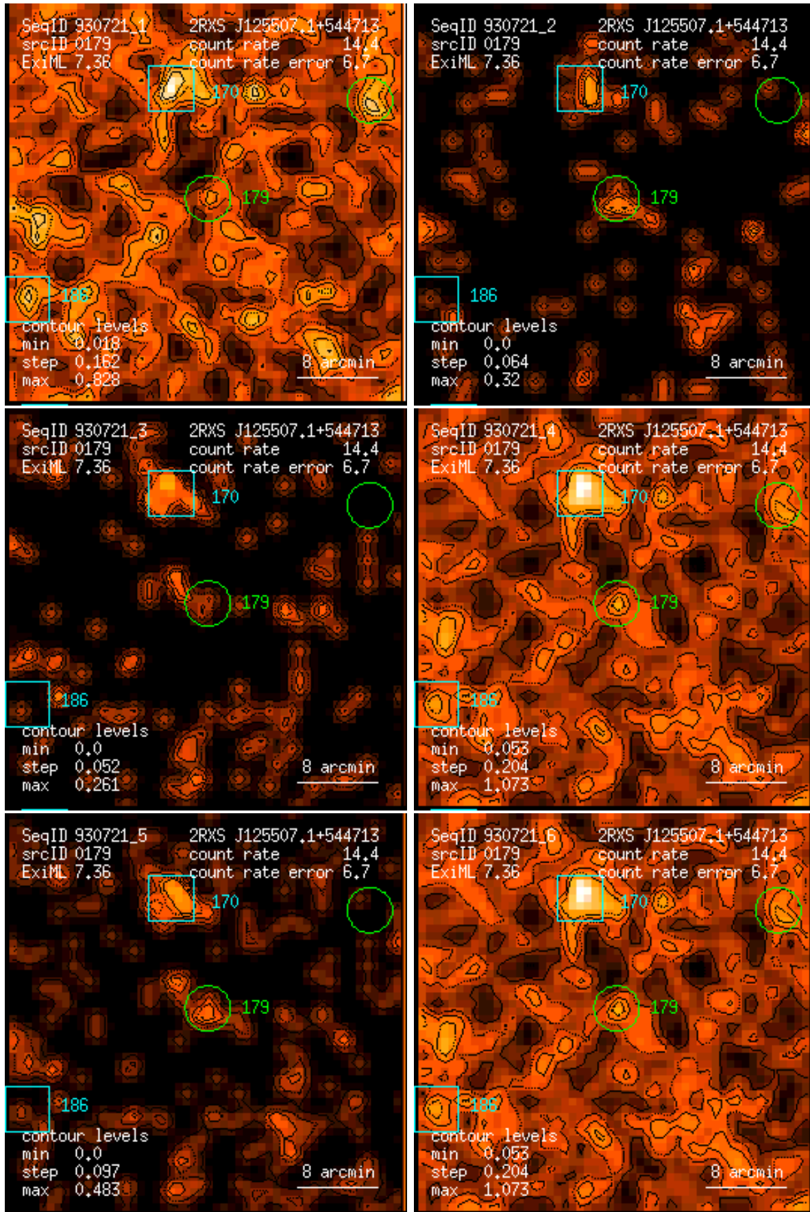
Figure 179: RASS 930721: detection 0179: band rate images, Gaussian filter: (1) PSPC channels 11 – 41, (2) 52 – 90, (3) 91 – 201, (4) 11 – 235, (5) 52 – 201, (6) 11 – 201. Broad band rates in counts/ks. Band rate contour levels in counts/ks/arcmin 2 .
