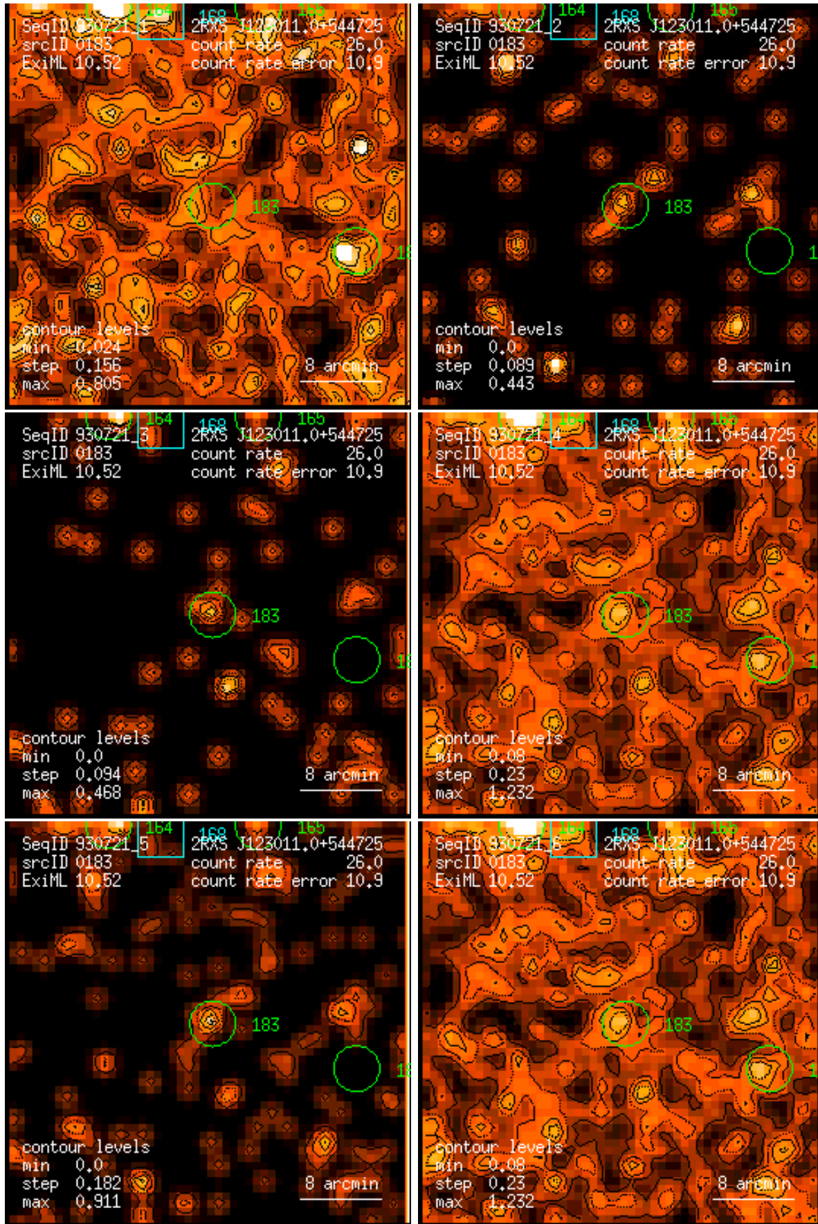
Figure 183: RASS 930721: detection 0183: band rate images, Gaussian filter: (1) PSPC channels 11 – 41, (2) 52 – 90, (3) 91 – 201, (4) 11 – 235, (5) 52 – 201, (6) 11 – 201. Broad band rates in counts/ks. Band rate contour levels in counts/ks/arcmin 2 .
